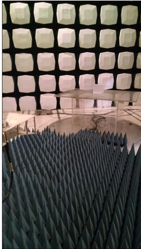
Photograph 3. Radiated Spurious Emissions, Test Setup, Above 1 GHz
