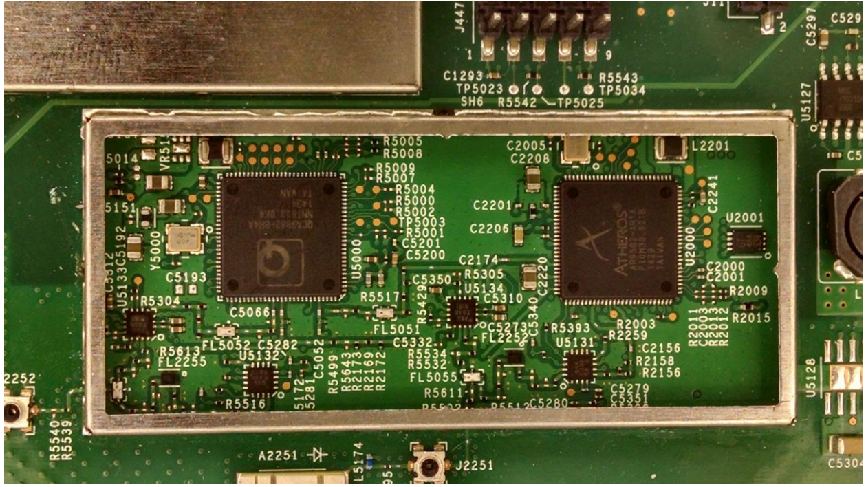
PCB assembly with ATHLETOS 3216 IC and various components.
