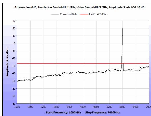
Plot 34. Radiated Spurious Emissions, 5785 MHz, 802.11n 20 MHz, 1 GHz – 7 GHz
