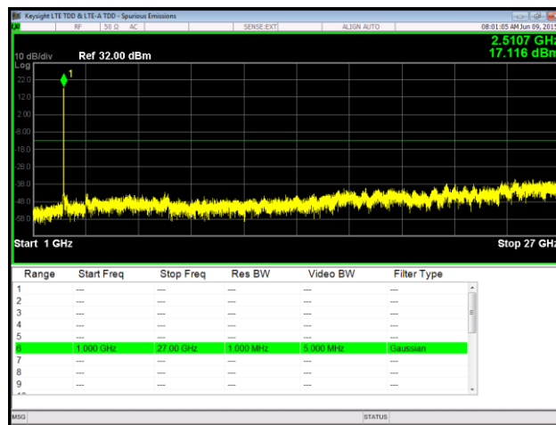
Plot 122. Spurious Emissions at Antenna Terminal, QPSK, Low Channel, Port 2, 1 GHz – 27 GHz
