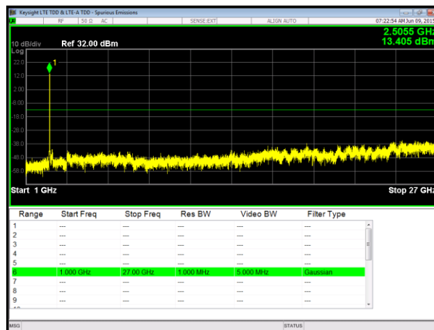
Plot 104. Spurious Emissions at Antenna Terminal, 64QAM, Low Channel, Port 1, 1 GHz – 27 GHz
