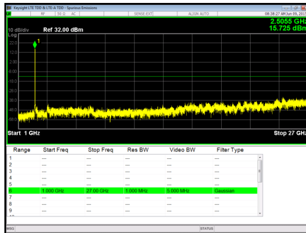
Plot 98. Spurious Emissions at Antenna Terminal, 16QAM, Low Channel, Port 2, 1 GHz – 27 GHz
