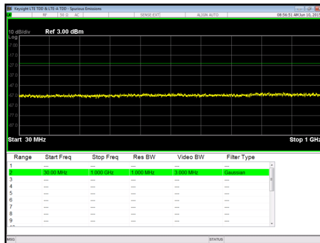
Plot 78. Spurious Emissions at Antenna Terminal, 16QAM, High Channel, Port 2, 30 MHz – 1 GHz, RBW
