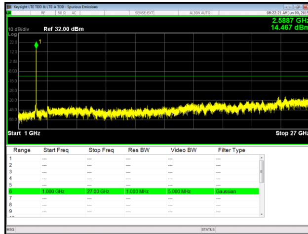
Plot 112. Spurious Emissions at Antenna Terminal, 64QAM, Mid Channel, Port 2, 1 GHz – 27 GHz
