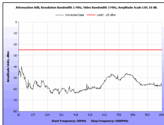
Plot 69. Radiated Spurious Emissions, QPSK, Mid Channel, Port 2, 30 MHz – 1 GHz
