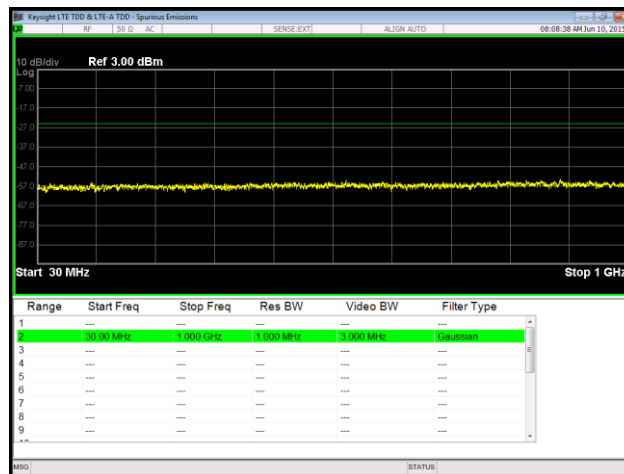
Plot 81. Spurious Emissions at Antenna Terminal, 64QAM, High Channel, Port 1, 30 MHz – 1 GHz, RBW
