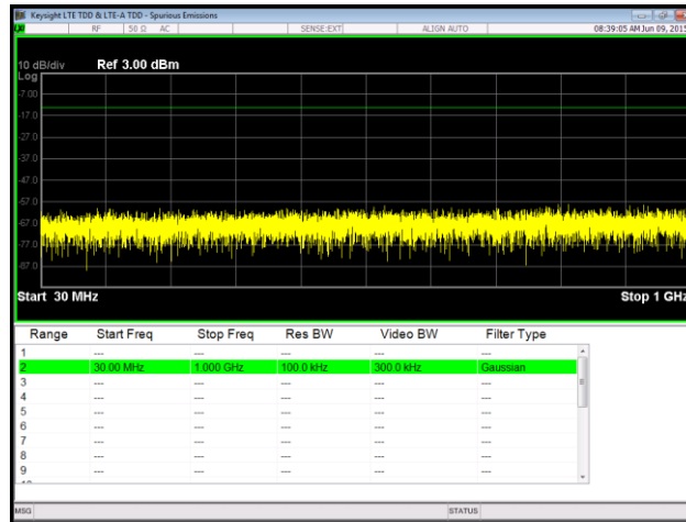
Plot 97. Spurious Emissions at Antenna Terminal, 16QAM, Low Channel, Port 2, 30 MHz – 1 GHz
