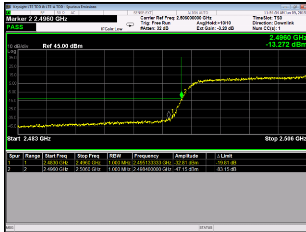
Plot 129. Conducted Band Edge, 16QAM, Low Channel, Port 2
