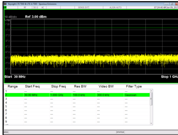
Plot 103. Spurious Emissions at Antenna Terminal, 64QAM, Low Channel, Port 1, 30 MHz – 1 GHz
