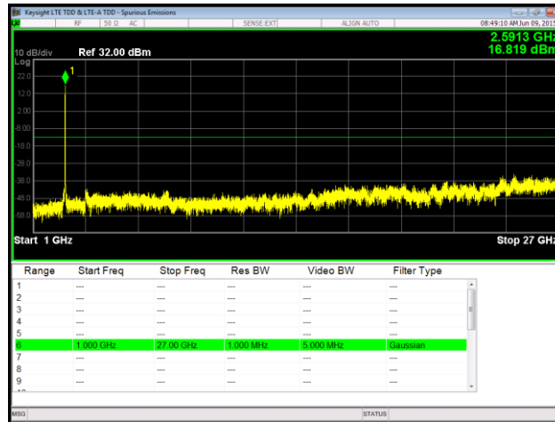
Plot 100. Spurious Emissions at Antenna Terminal, 16QAM, Mid Channel, Port 2, 1 GHz – 27 GHz
