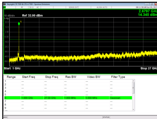
Plot 126. Spurious Emissions at Antenna Terminal, QPSK, High Channel, Port 2, 1 GHz – 27 GHz
