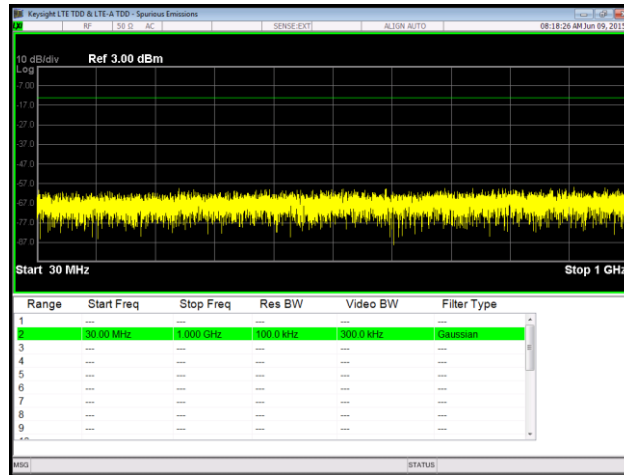
Plot 109. Spurious Emissions at Antenna Terminal, 64QAM, Low Channel, Port 2, 30 MHz – 1 GHz
