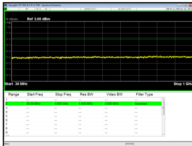
Plot 90. Spurious Emissions at Antenna Terminal, QPSK, High Channel, Port 2, 30 MHz – 1 GHz, RBW
