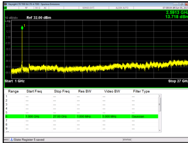
Plot 118. Spurious Emissions at Antenna Terminal, QPSK, Mid Channel, Port 1, 1 GHz – 27 GHz
