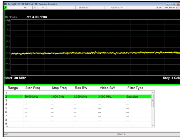
Plot 88. Spurious Emissions at Antenna Terminal, QPSK, Low Channel, Port 2, 30 MHz – 1 GHz, RBW
