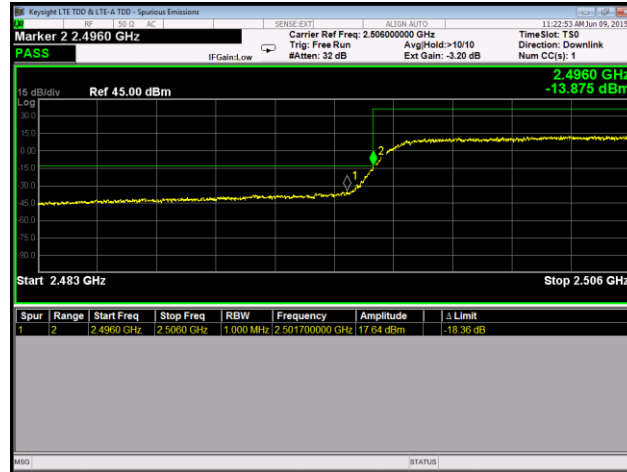
Plot 127. Conducted Band Edge, 16QAM, Low Channel, Port 1
