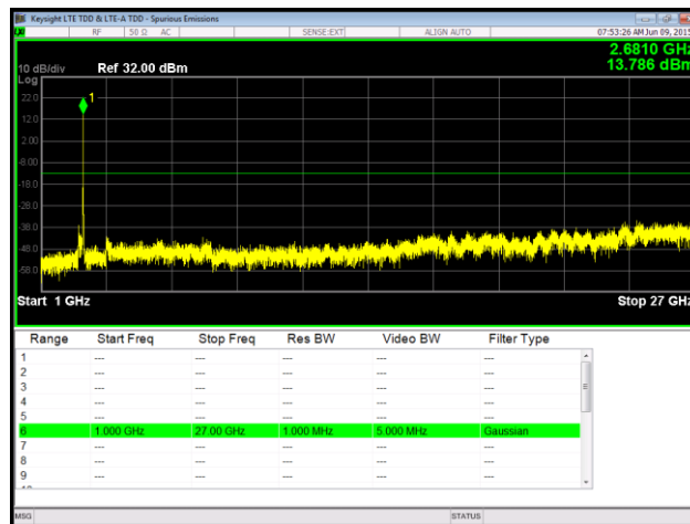
Plot 96. Spurious Emissions at Antenna Terminal, 16QAM, High Channel, Port 1, 1 GHz – 27 GHz
