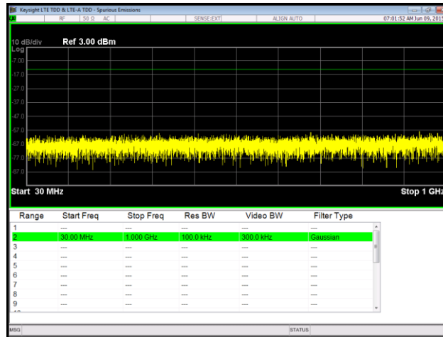
Plot 115. Spurious Emissions at Antenna Terminal, QPSK, Low Channel, Port 1, 30 MHz – 1 GHz
