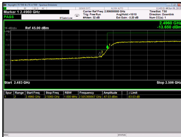
Plot 137. Conducted Band Edge, QPSK, Low Channel, Port 2
