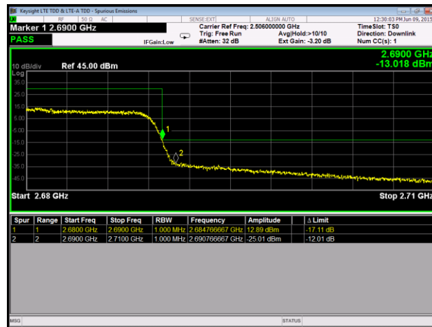
Plot 128. Conducted Band Edge, 16QAM, High Channel, Port 1
