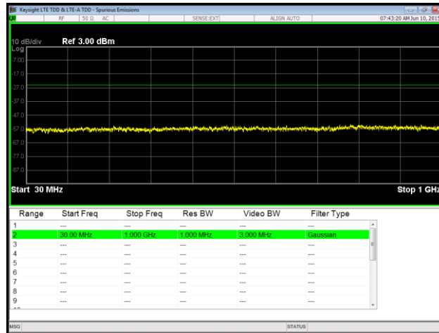
Plot 73. Spurious Emissions at Antenna Terminal, 16QAM, Low Channel, Port 1, 30 MHz – 1 GHz, RBW
