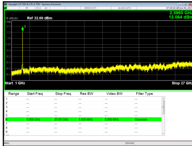
Plot 106. Spurious Emissions at Antenna Terminal, 64QAM, Mid Channel, Port 1, 1 GHz – 27 GHz
