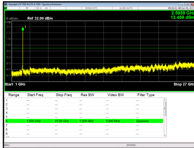
Plot 124. Spurious Emissions at Antenna Terminal, QPSK, Mid Channel, Port 2, 1 GHz – 27 GHz
