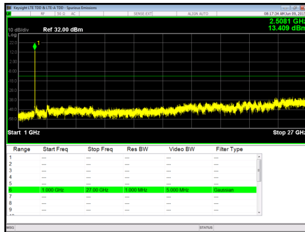
Plot 110. Spurious Emissions at Antenna Terminal, 64QAM, Low Channel, Port 2, 1 GHz – 27 GHz
