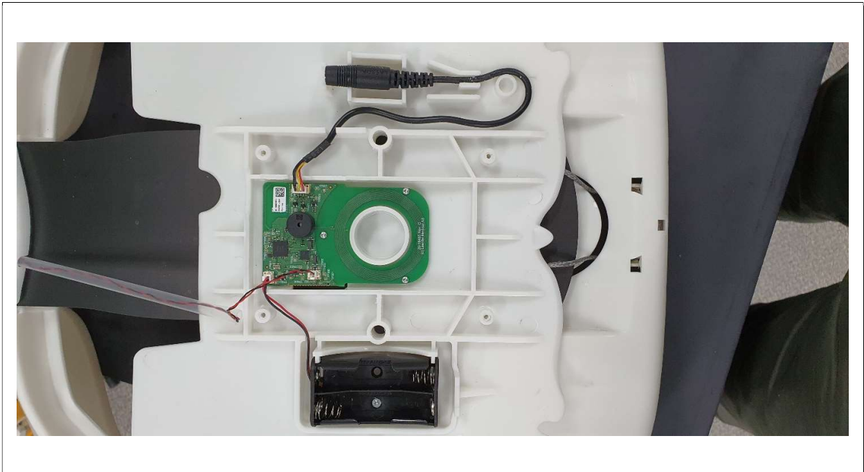
Overview
