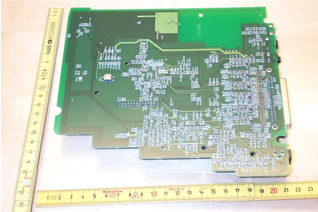
Solder-side of printed circuit board.
