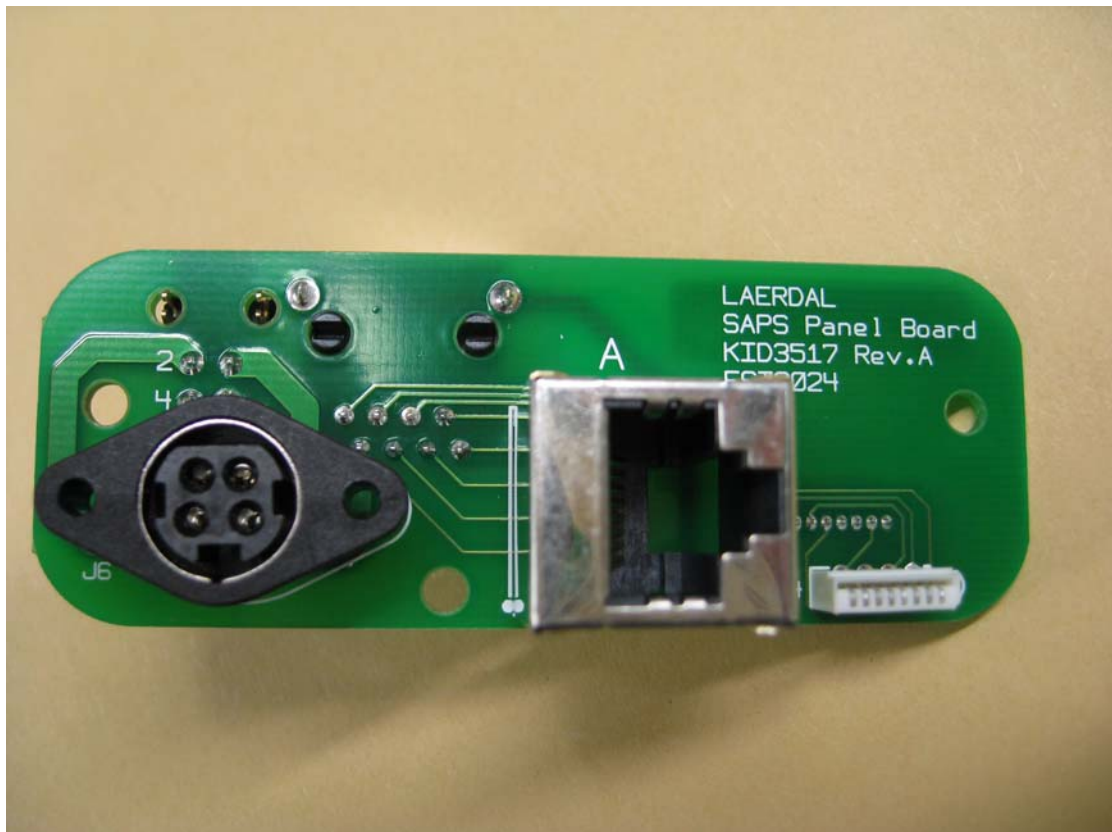
SAPS Panel board FST2024
