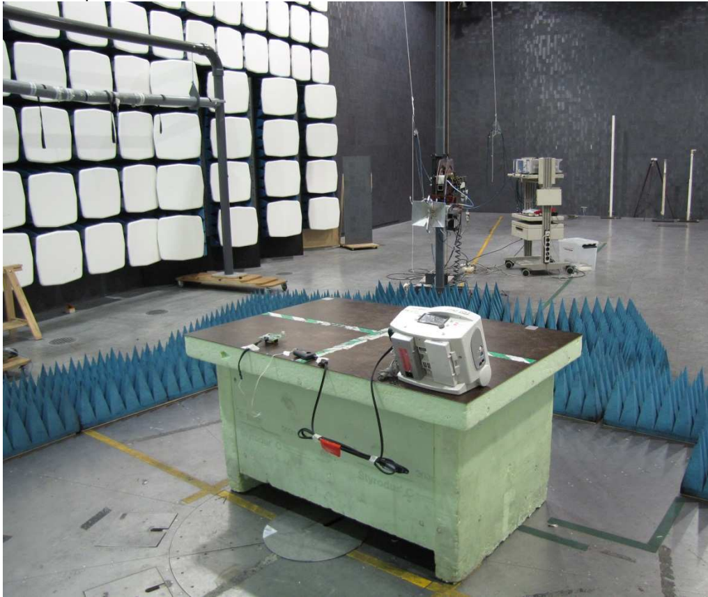
Test set up radiated emission 18 GHz – 26.5 GHz
