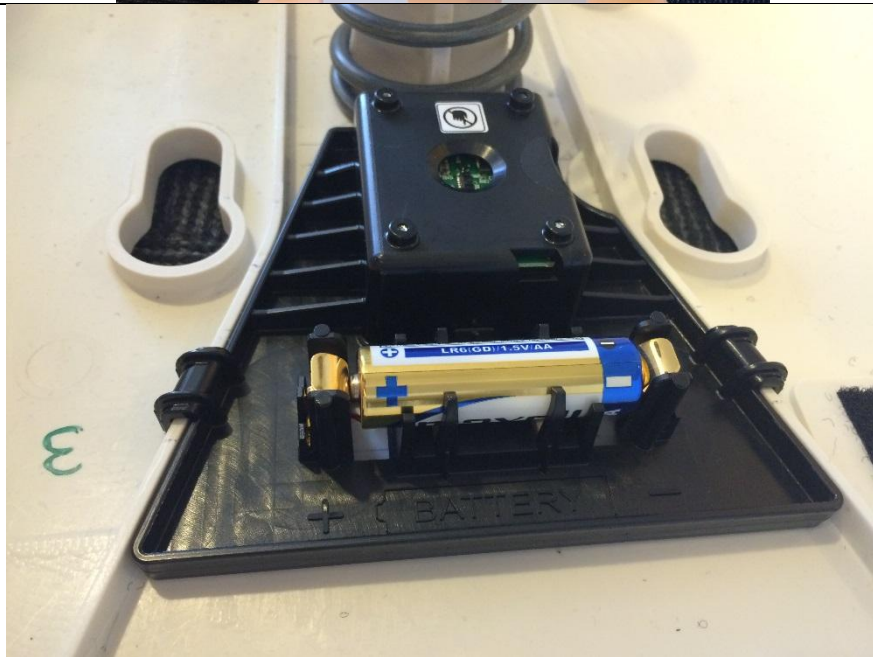
Picture 6 Little Anne QCPR Sensor – “Front view”
