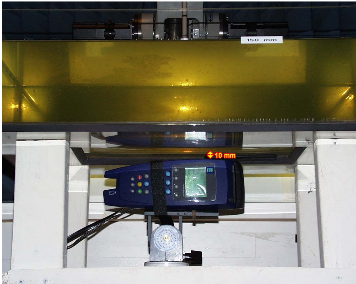
< Right of EUT faced toward phantom at 10 mm separation, swivel antenna 180°(fully extended) >
