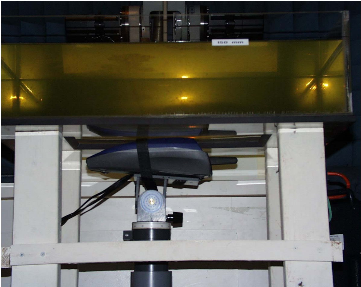
< Prescan - Front side of EUT faced toward phantom and in contact, swivel antenna 180°(fully extended) >
