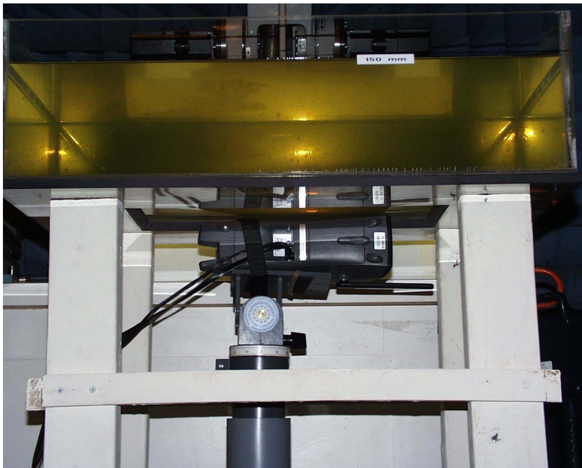
< Prescan - Left side of EUT faced toward phantom and in contact, swivel antenna 180°(fully extended) >
