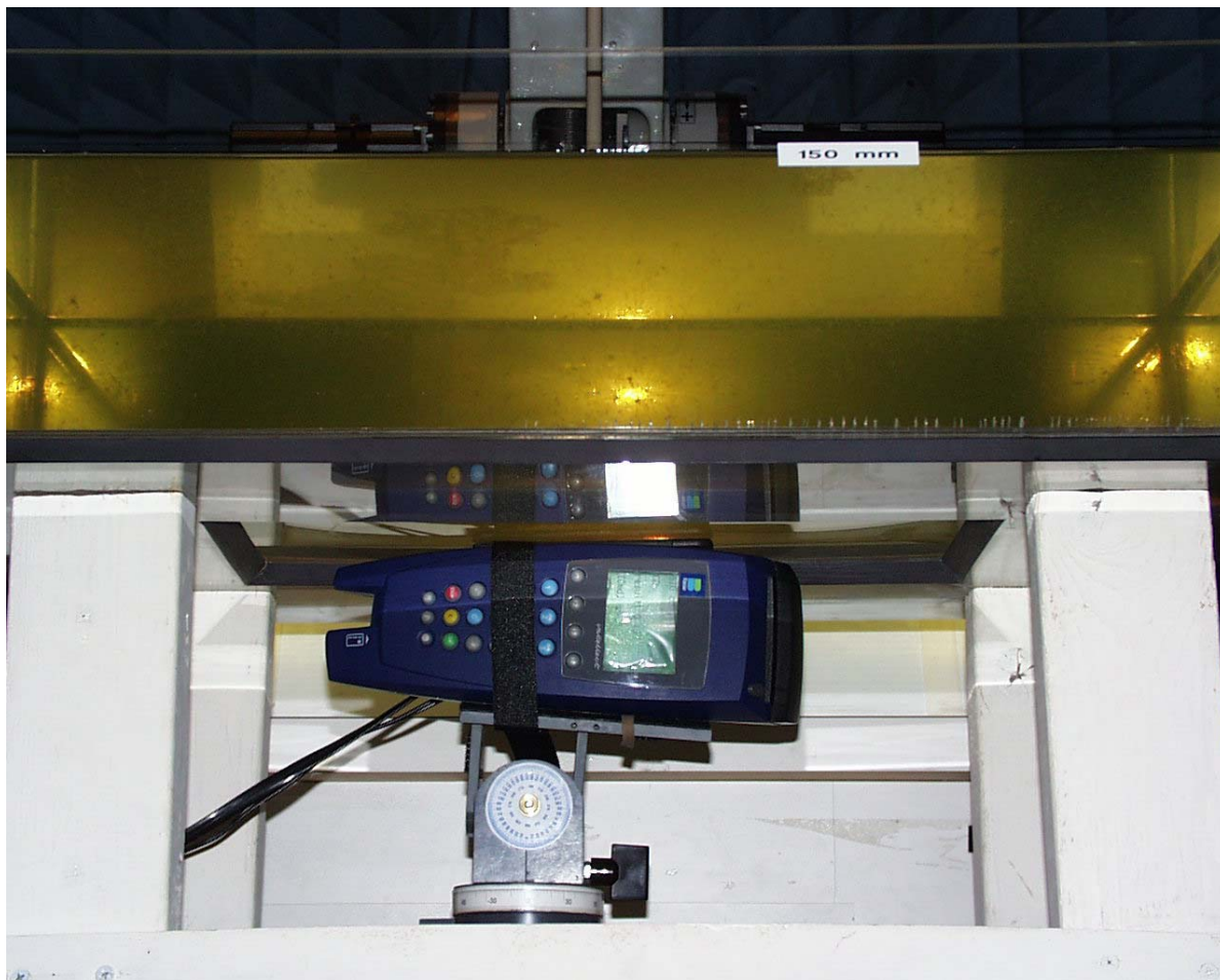
< Prescan – Right of EUT faced toward phantom and in contact, swivel antenna 0, swivel antenna 0°(fully retracted) >
