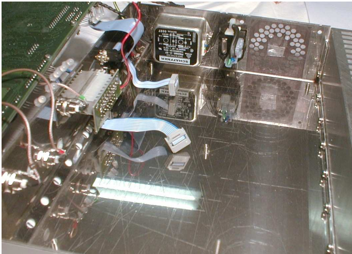
Detail view, right face
