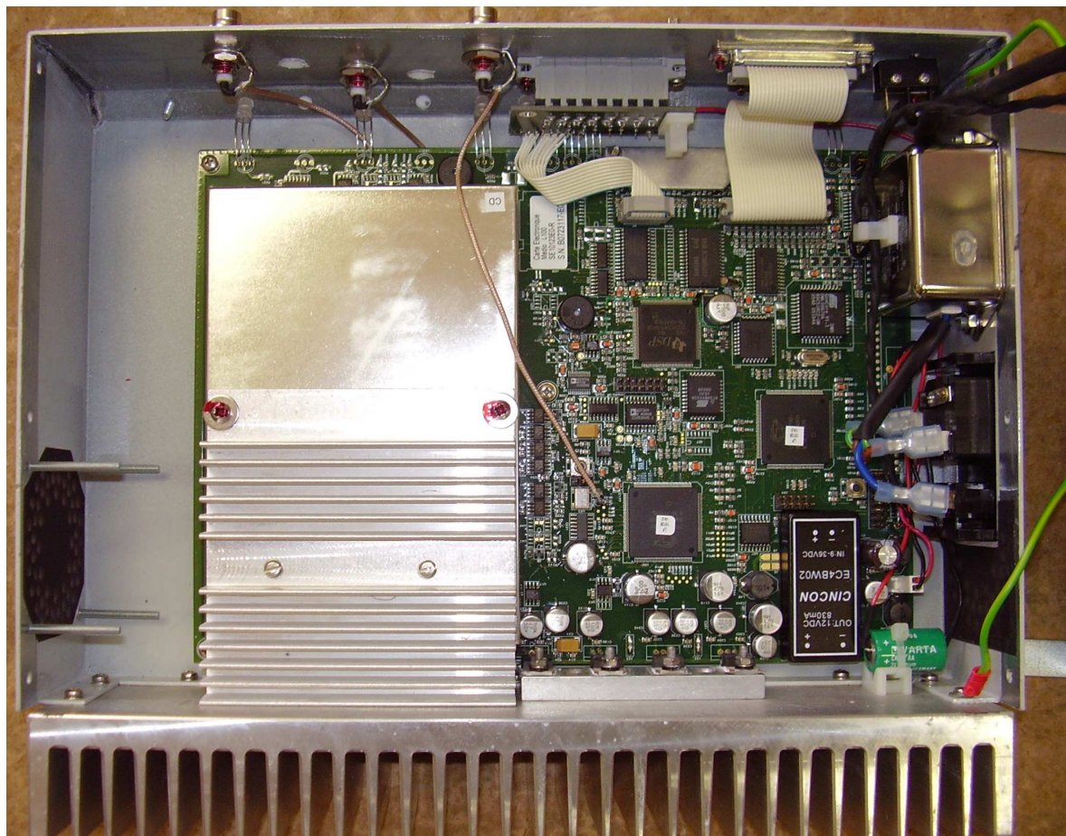
TR-L100 reader (Cover removed)
