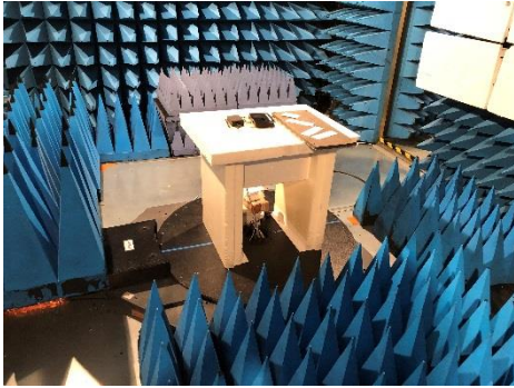
Test setup in anechoic chamber <1GHz (pre-characterization)
