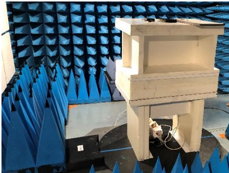
Test setup in anechoic chamber >1GHz (pre-characterization and characterization)
