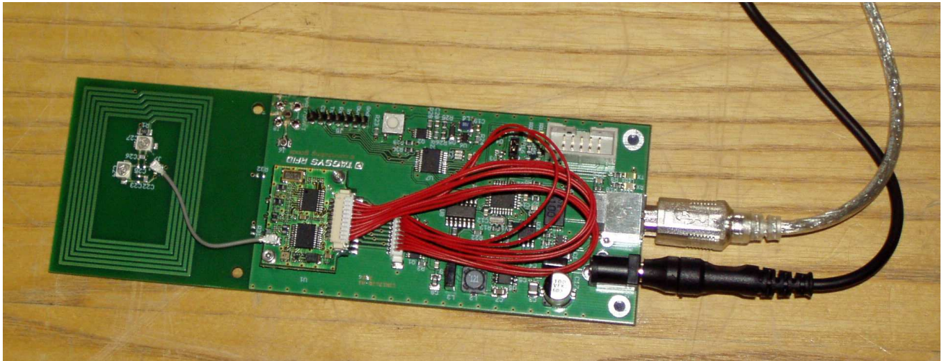
General view of the MEDIO S004 evaluation board
