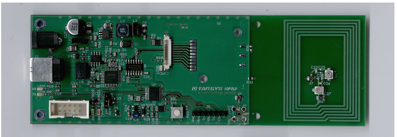
MEDIO S004 EVM board without RF module
