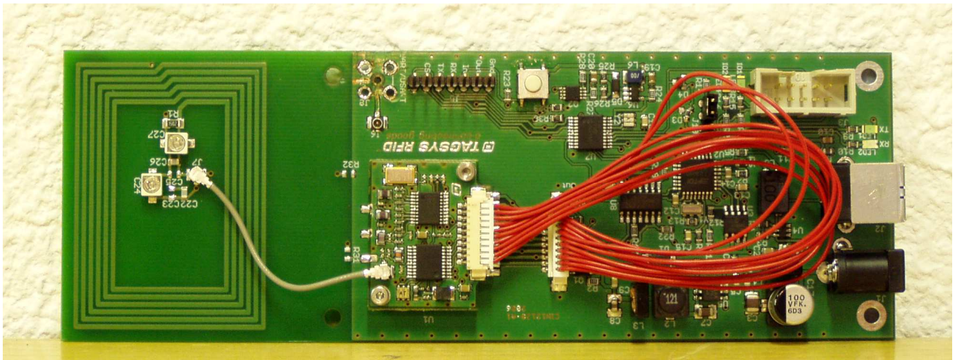
Upper side of the board
