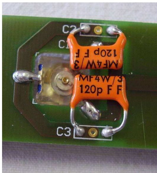
AERO-LB antenna (detail view)
