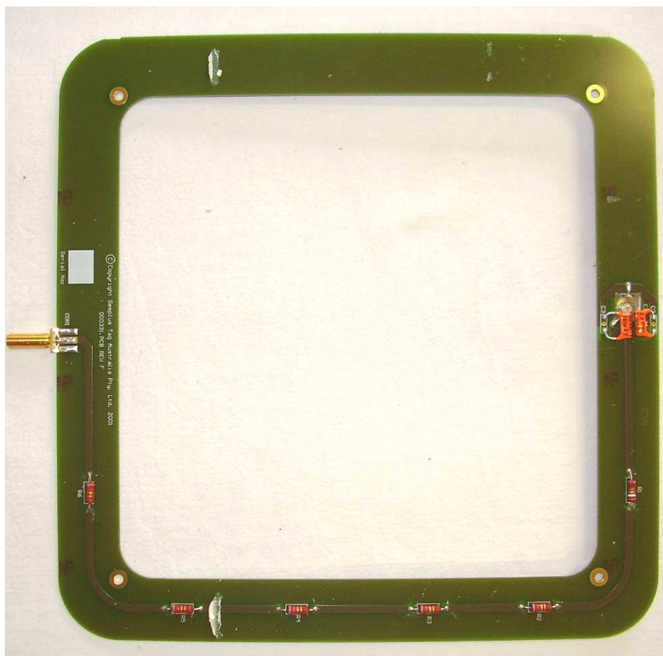
AERO-LB antenna
