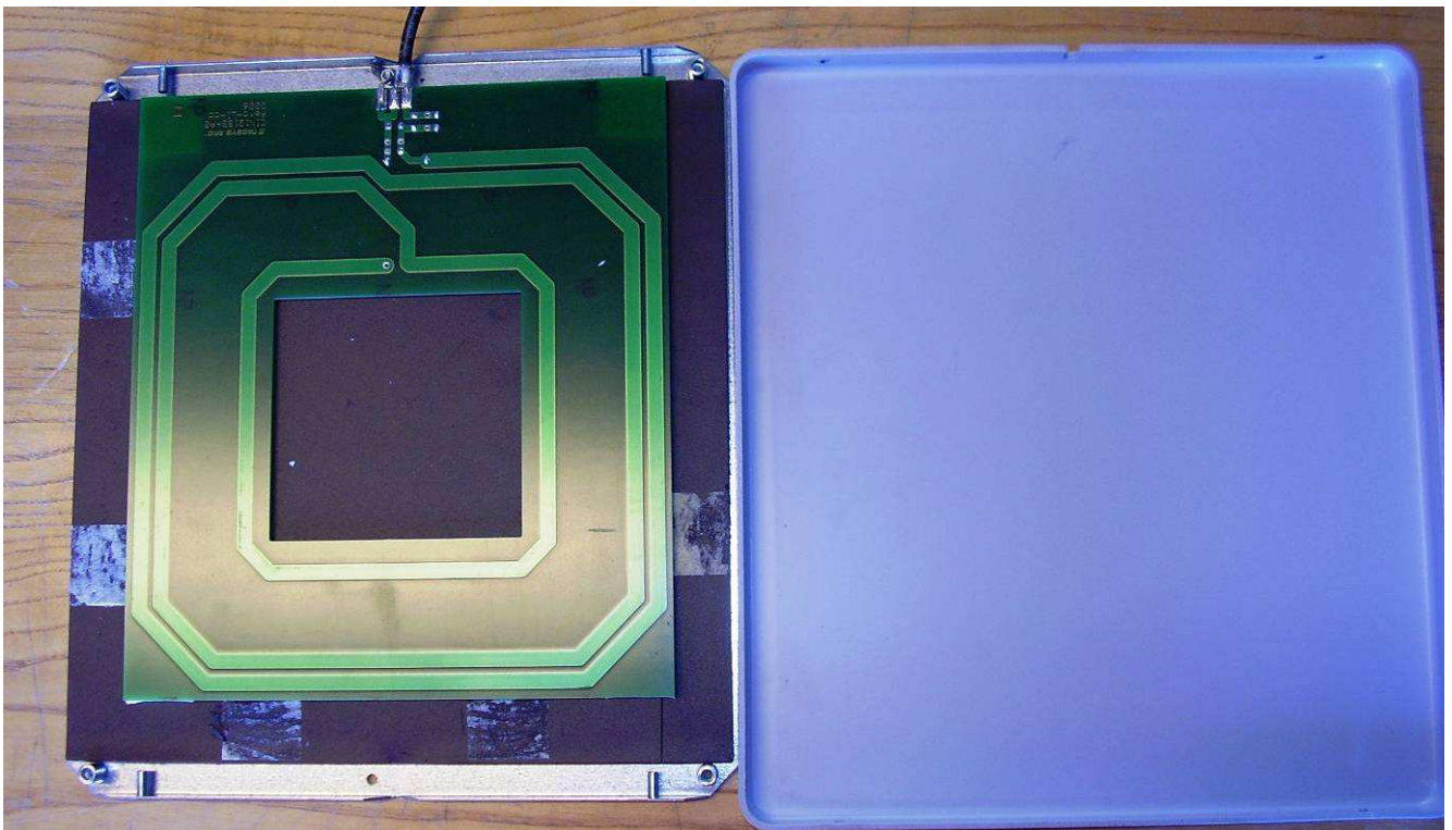
General view of the L-SA4 antenna
