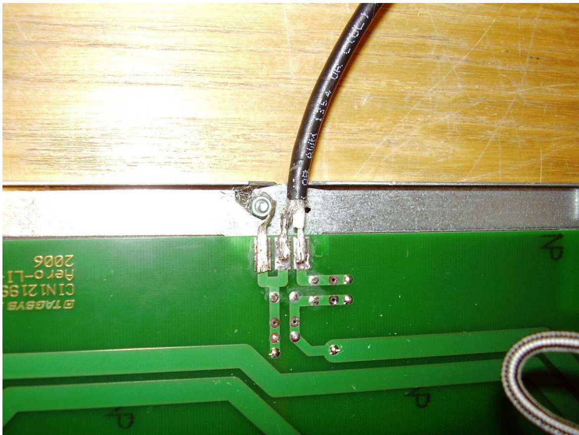
Detail view of the RF cable connection to PCB (L-SA4 antenna)
