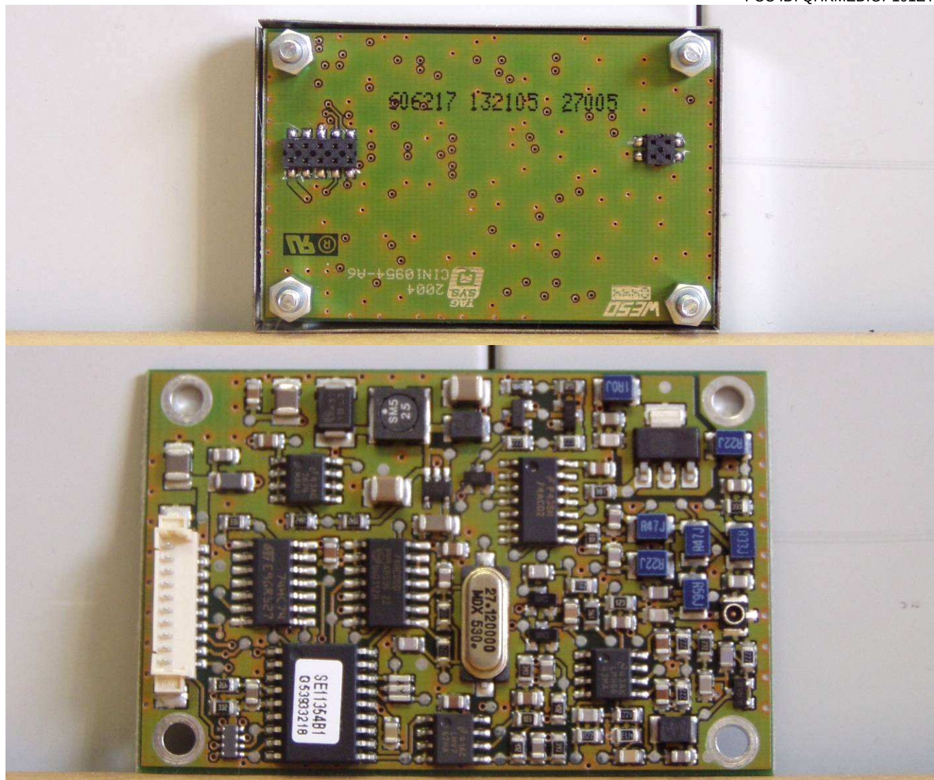
RF board
