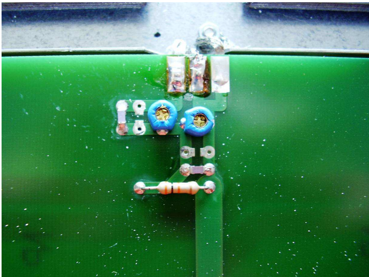
Component view (L-SA4 antenna)
