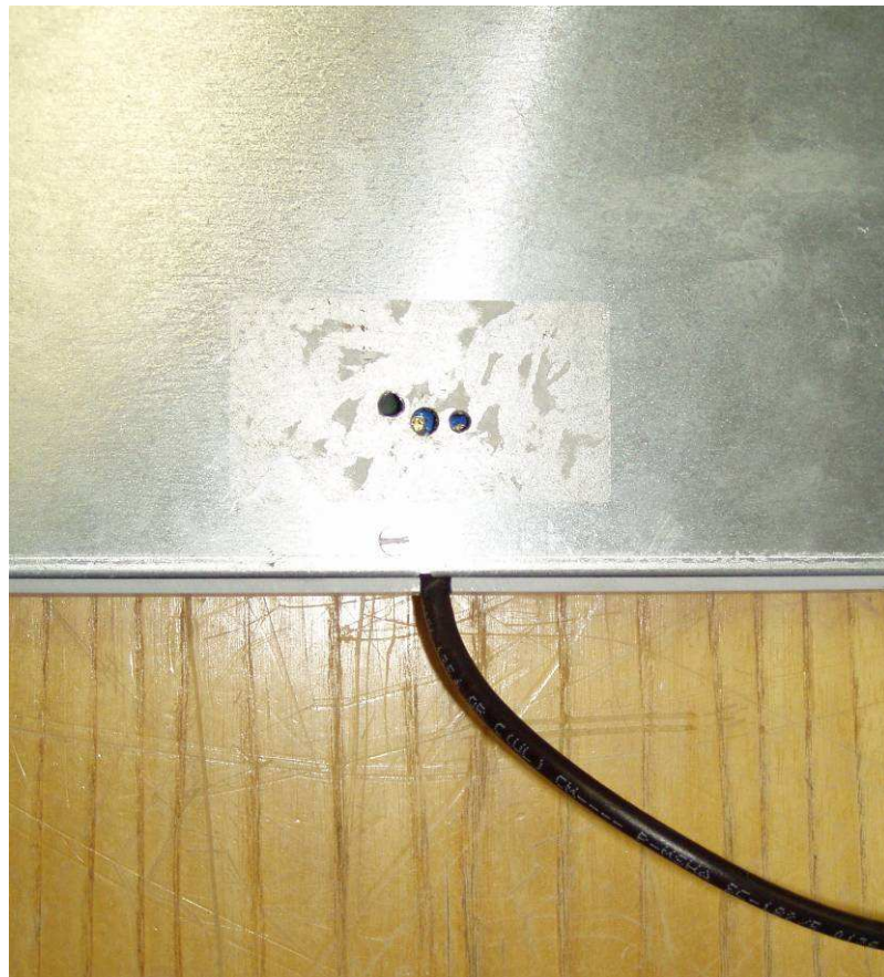
LSA-4 antenna
