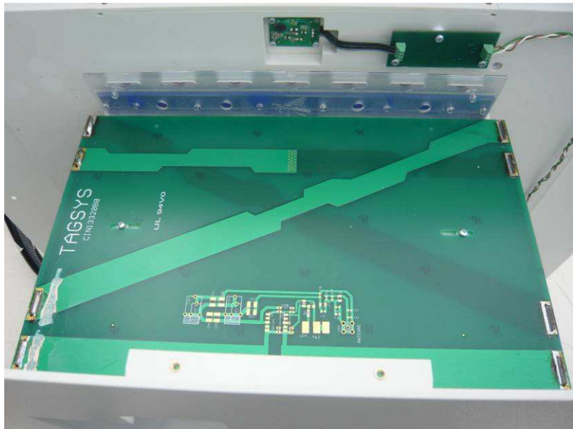
Top view with the detector
