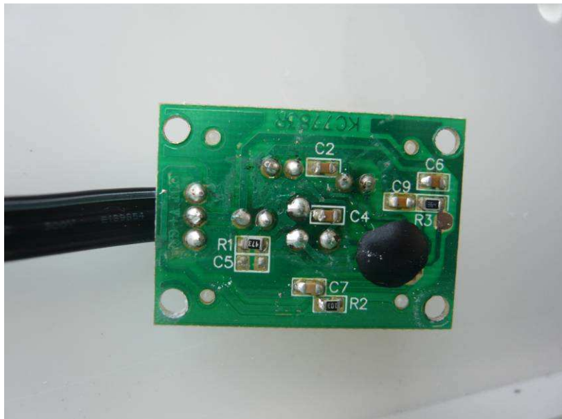
Detail views of the PCB detector
