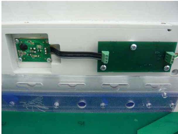
Top view with the detector
