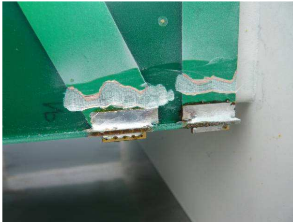
Modification for using just 2 antennas
