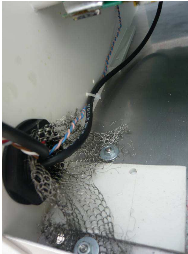
Detail view of output cables
