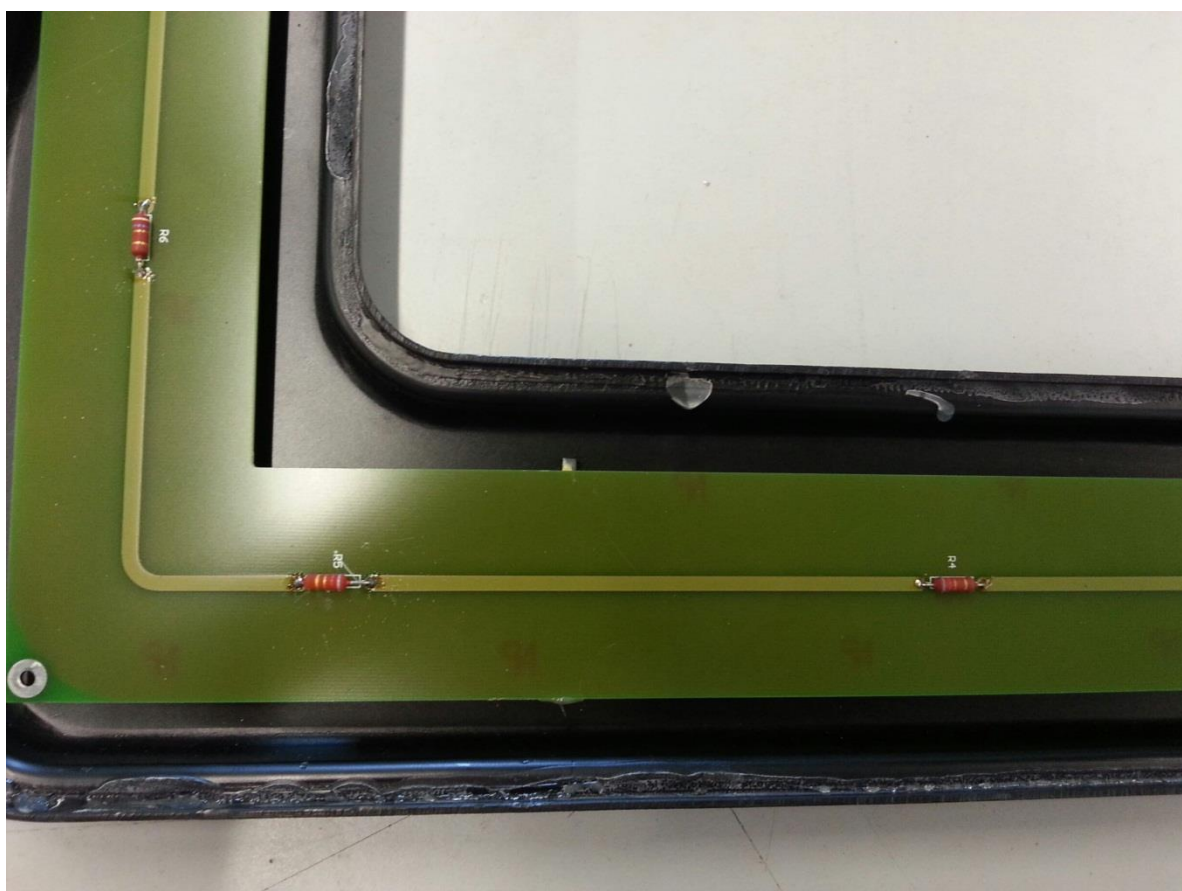
Detail views of AERO LC antenna
