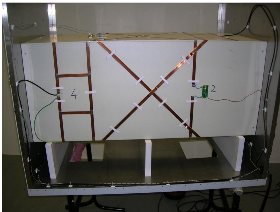
Detail views of Tunnel antenna
