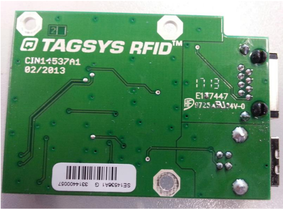
Detail views of USB and RS232 card
