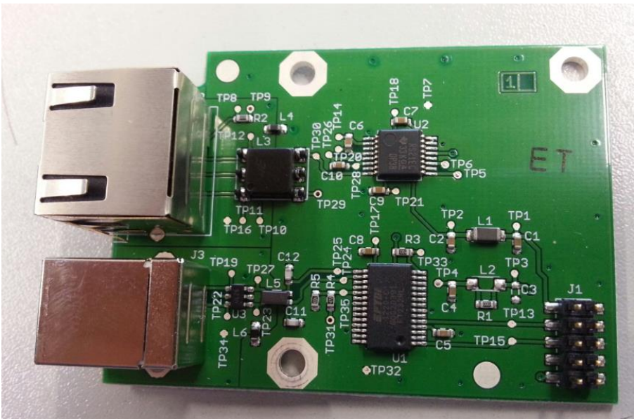
Detail views of USB and RS232 card
