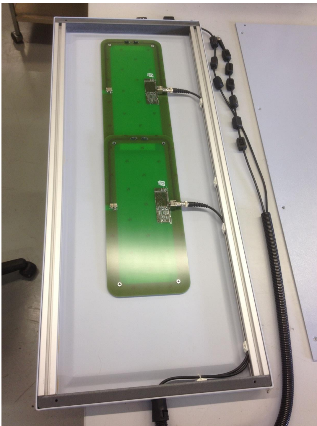
Detail views of TR-CAu antenna
