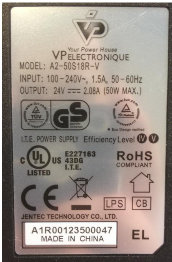
Views of VP ELECTRONIQUE power supply
