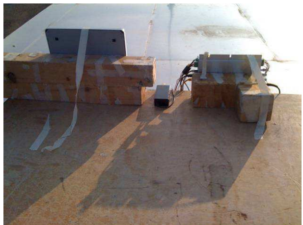
LSA4 Configuration
