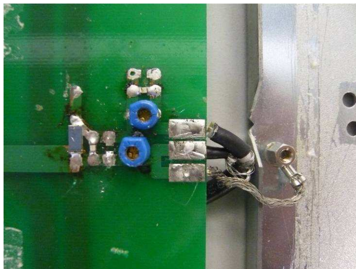
Detail views of LSA4 antenna
