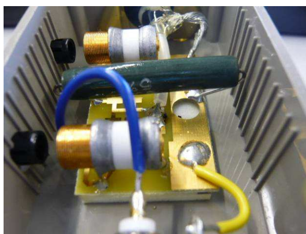
Detail views of MAT antenna
