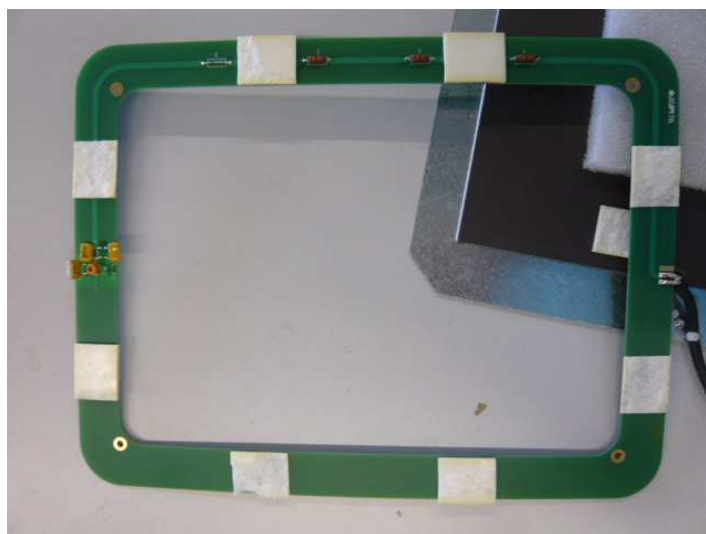
Detail views of LSA3 antenna
