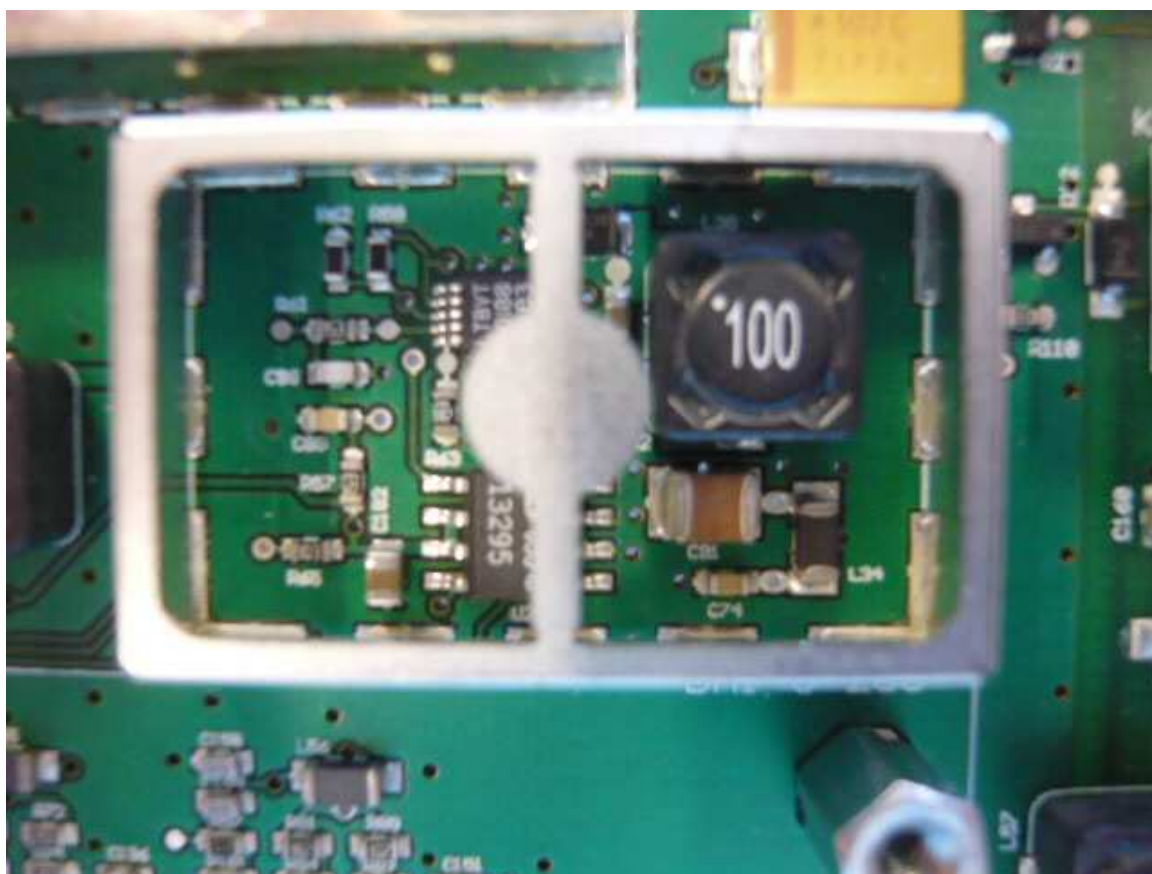
Views without shielding
