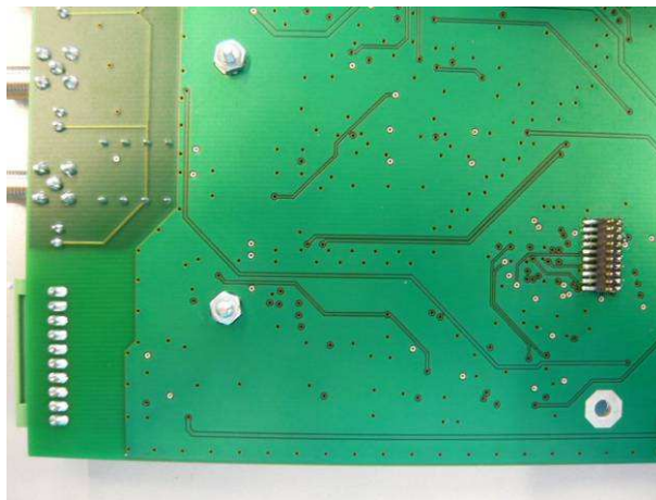
Views of other side
