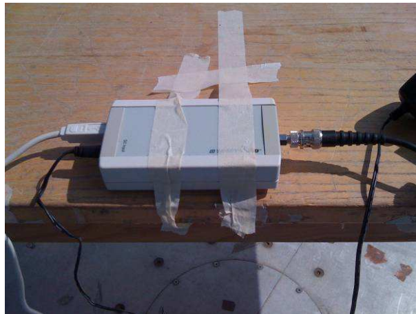
Radiated setup – LSA3 configuration
