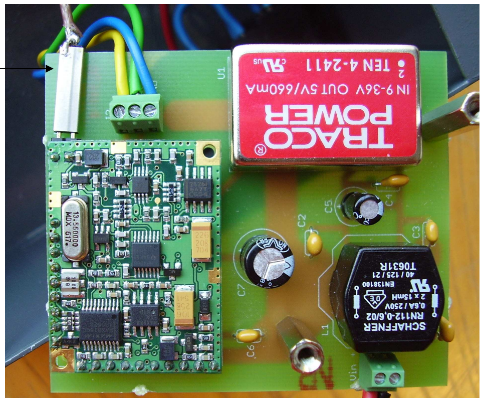
RF board with S002 module
