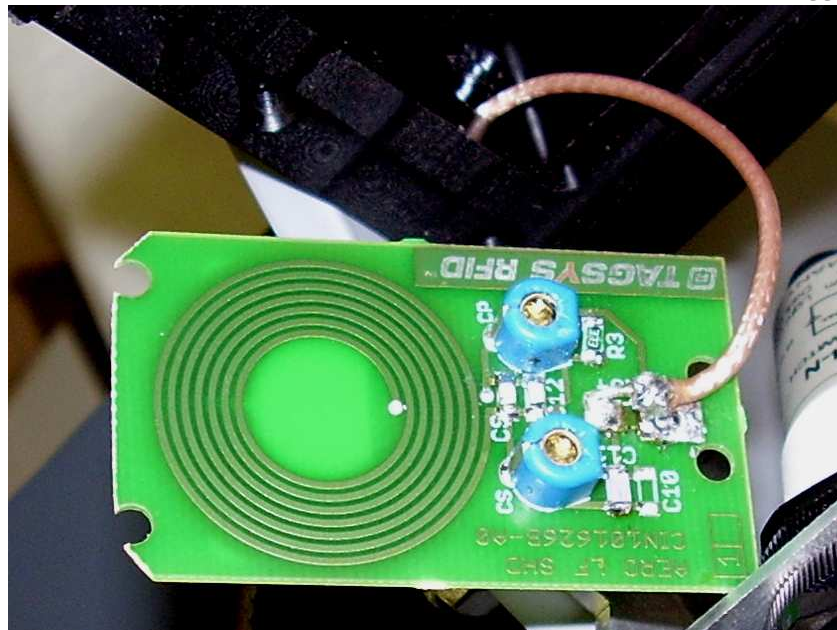
Detail view of RF cable soldering on antenna
