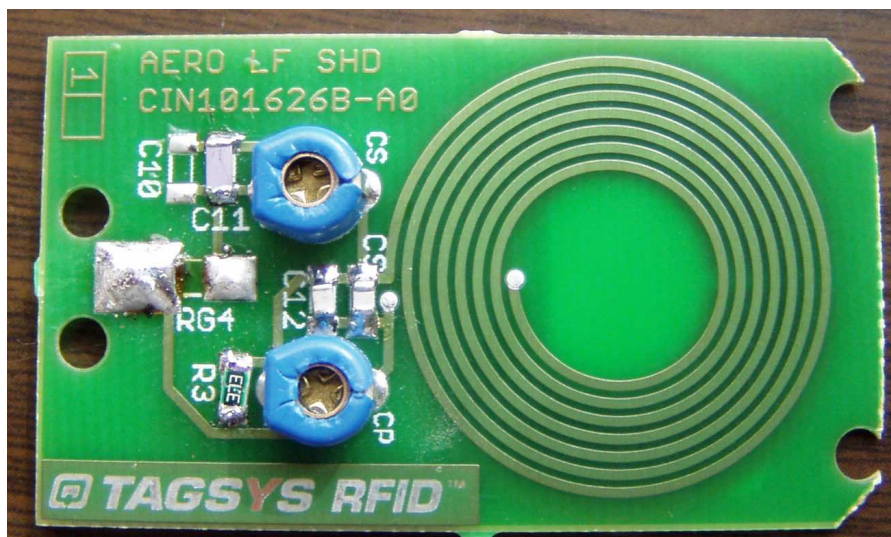
RF antenna
