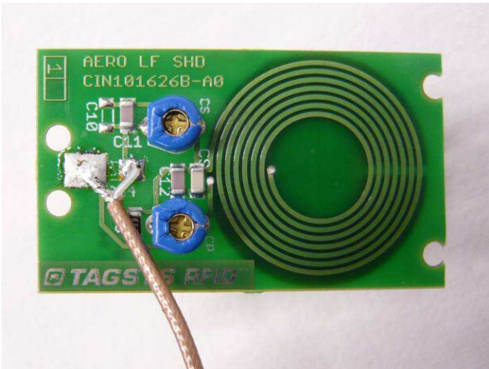
Bottom view of antenna
