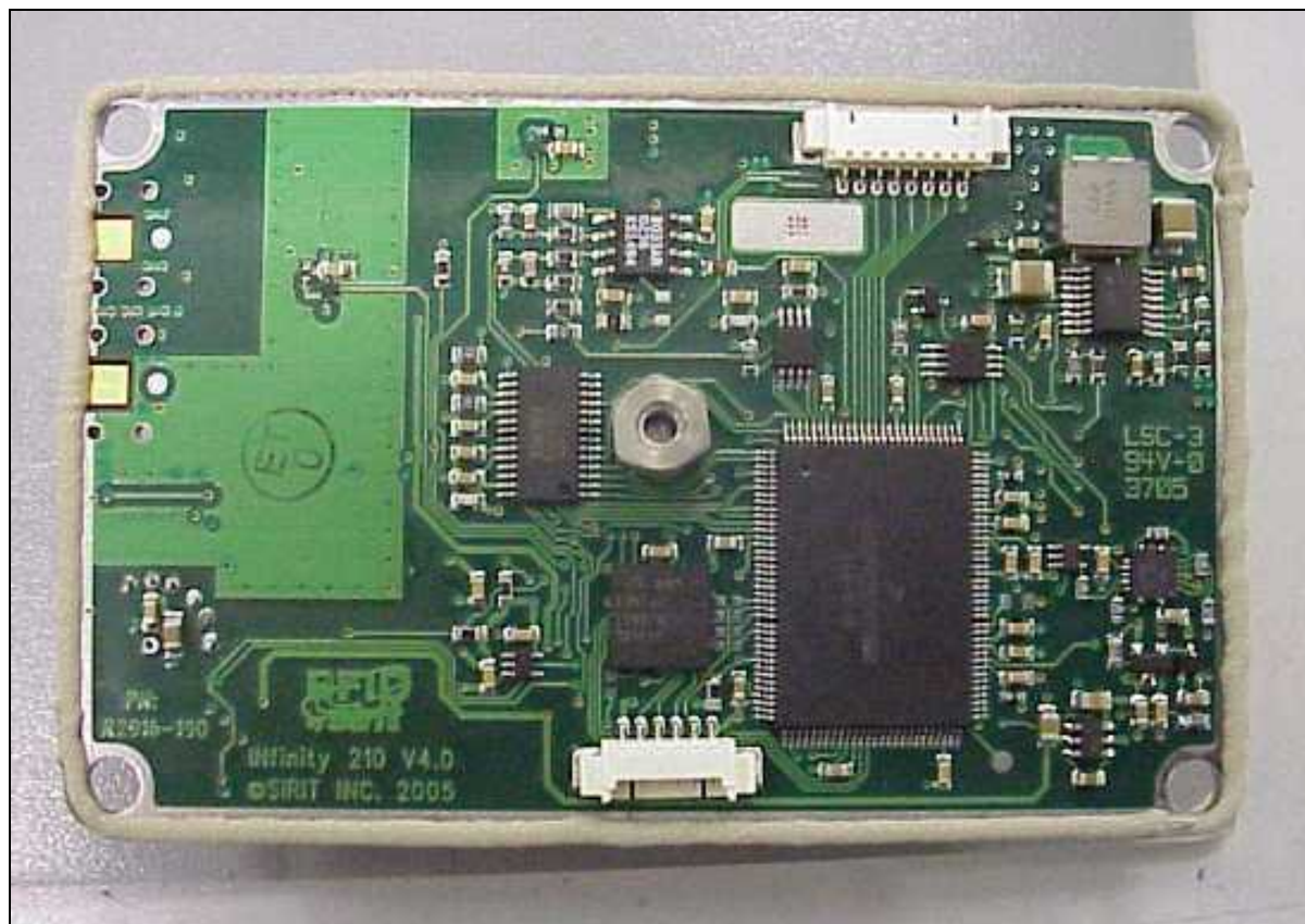
Bottom view
