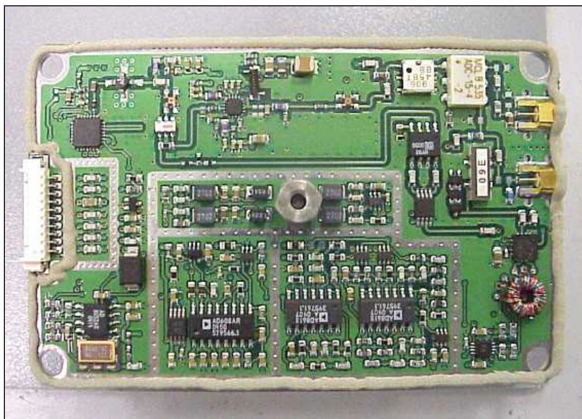
Top view
