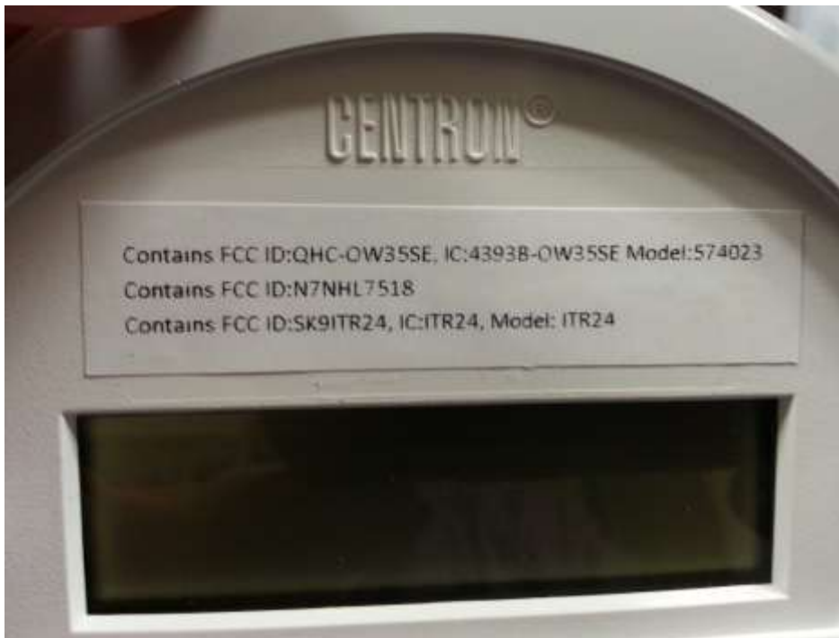
FCC & IC LABEL ON HOST METER
