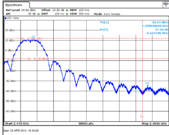
Figure 7.5.1.2-11: Upper Band-edge - 2475 MHz
