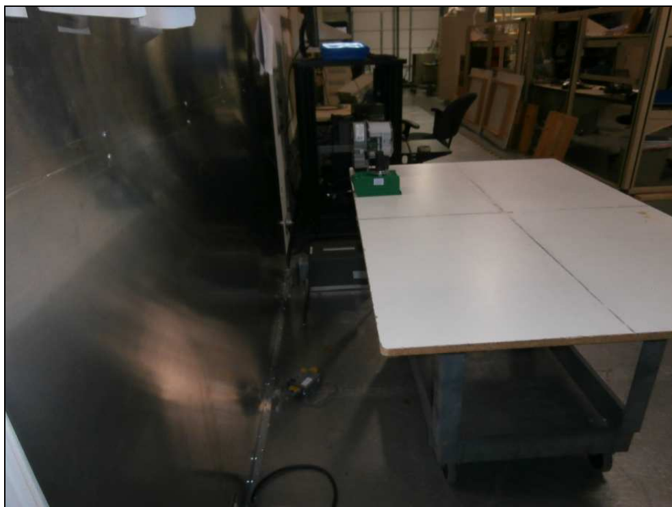
Figure 10: Conducted Emissions – 12S Meter Form – CDMA Modem External Antenna Option
