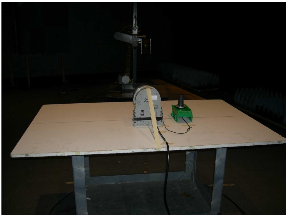
Figure 4: Radiated Emissions – 2S Meter Form – CDMA Modem External Antenna Option
