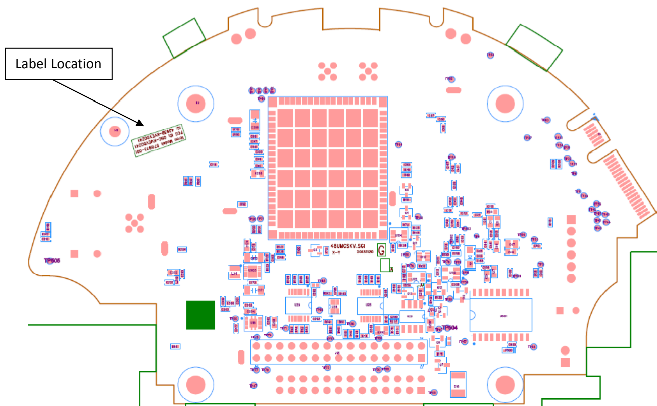
Kv2c-AMPZ FCC & IC Module Label Location
