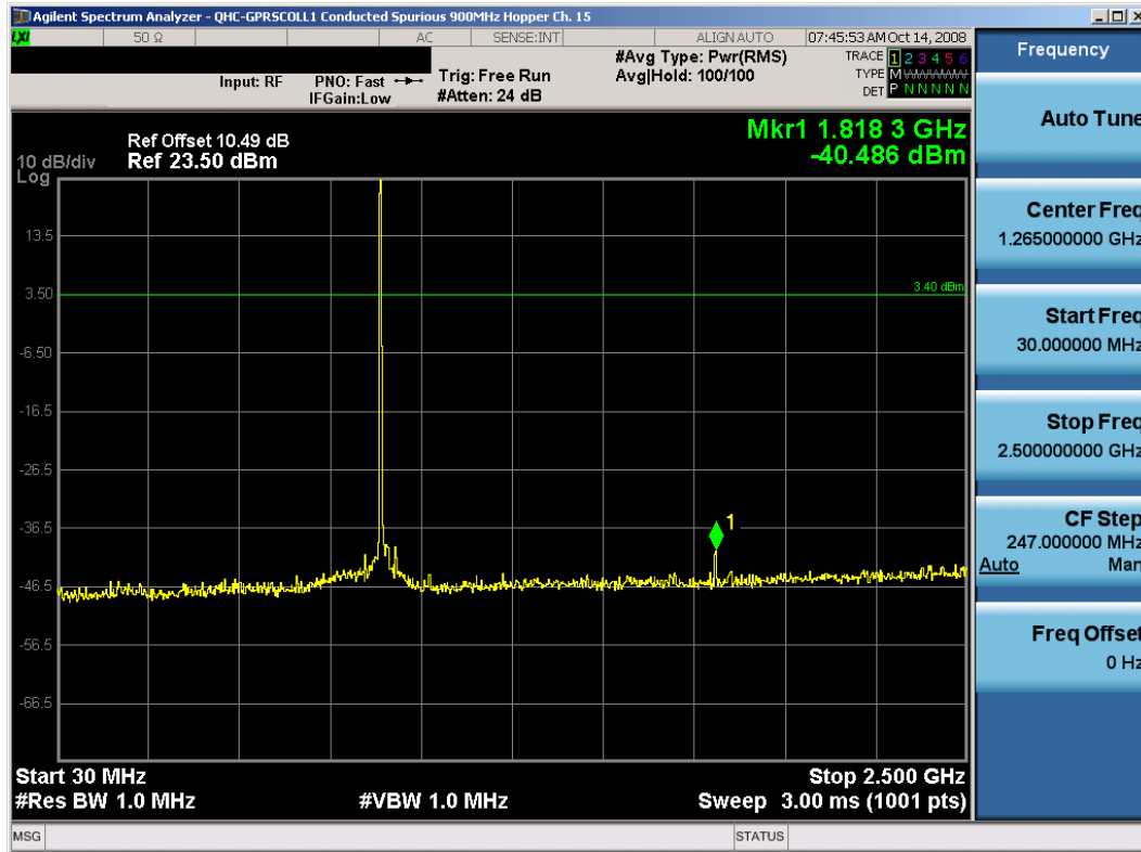
Plot 6-17. Conducted Spurious Plot (Ch. 15)
