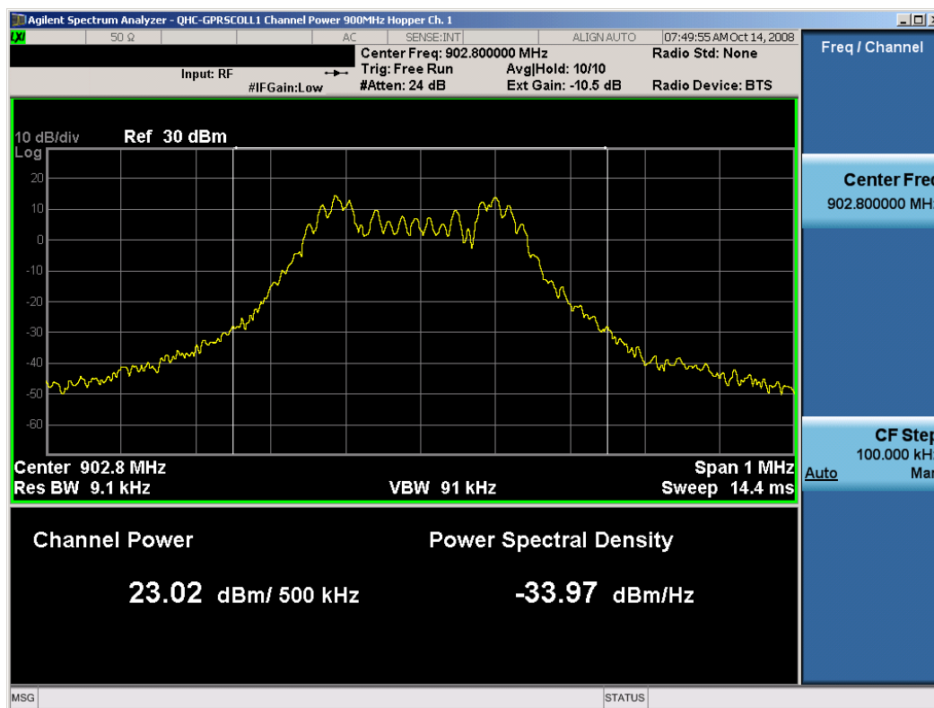
Plot 6-4. Conducted Output Power (Ch. 1)
