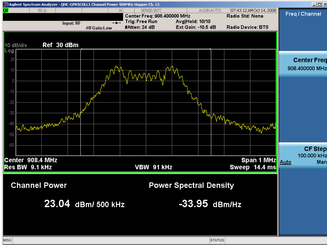
Plot 6-5. Conducted Output Power (Ch. 15)
