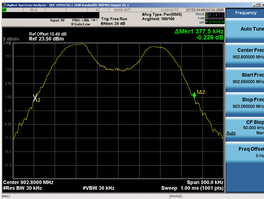
Plot 6-1. 20dB Bandwidth Plot (Ch. 1)
