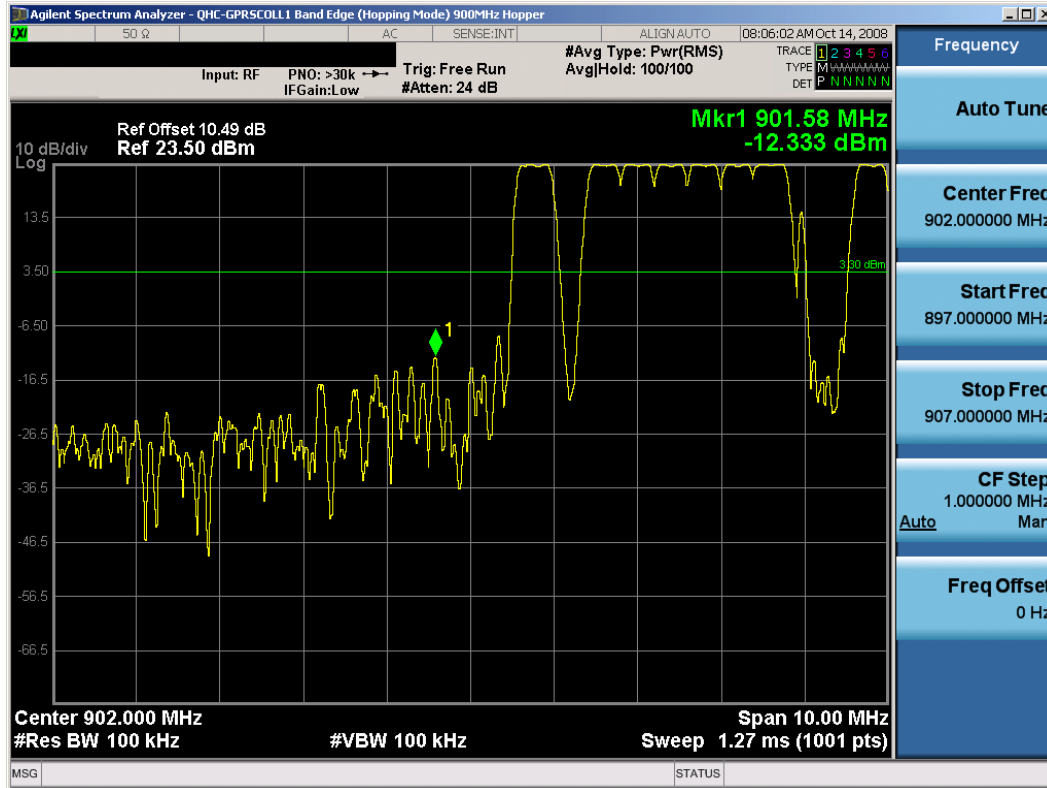
Plot 6-9. Lower Band Edge Plot (Hopping Mode) (Ch. 1)
