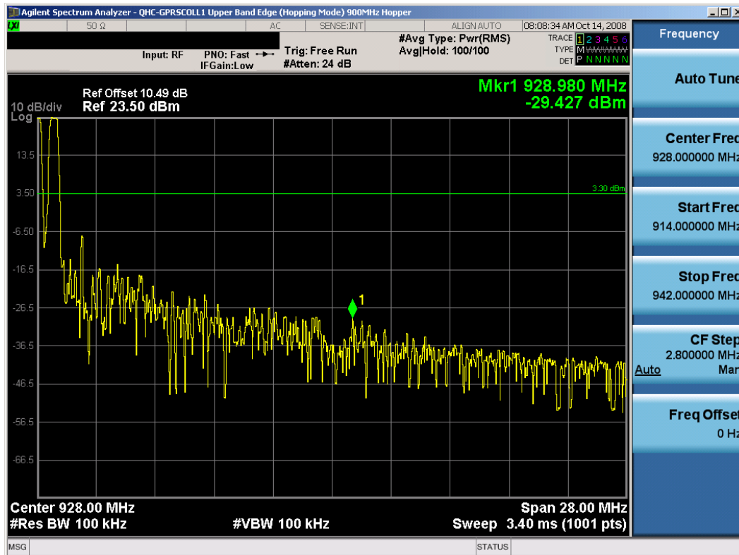
Plot 6-10. Upped Band Edge Plot (Hopping Mode) (Ch. 31)
