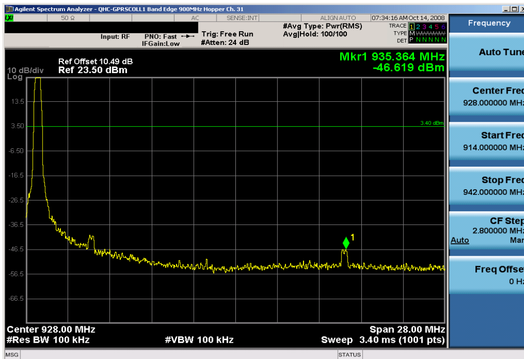
Plot 6-8. Upper Band Edge Plot (Ch. 31)
