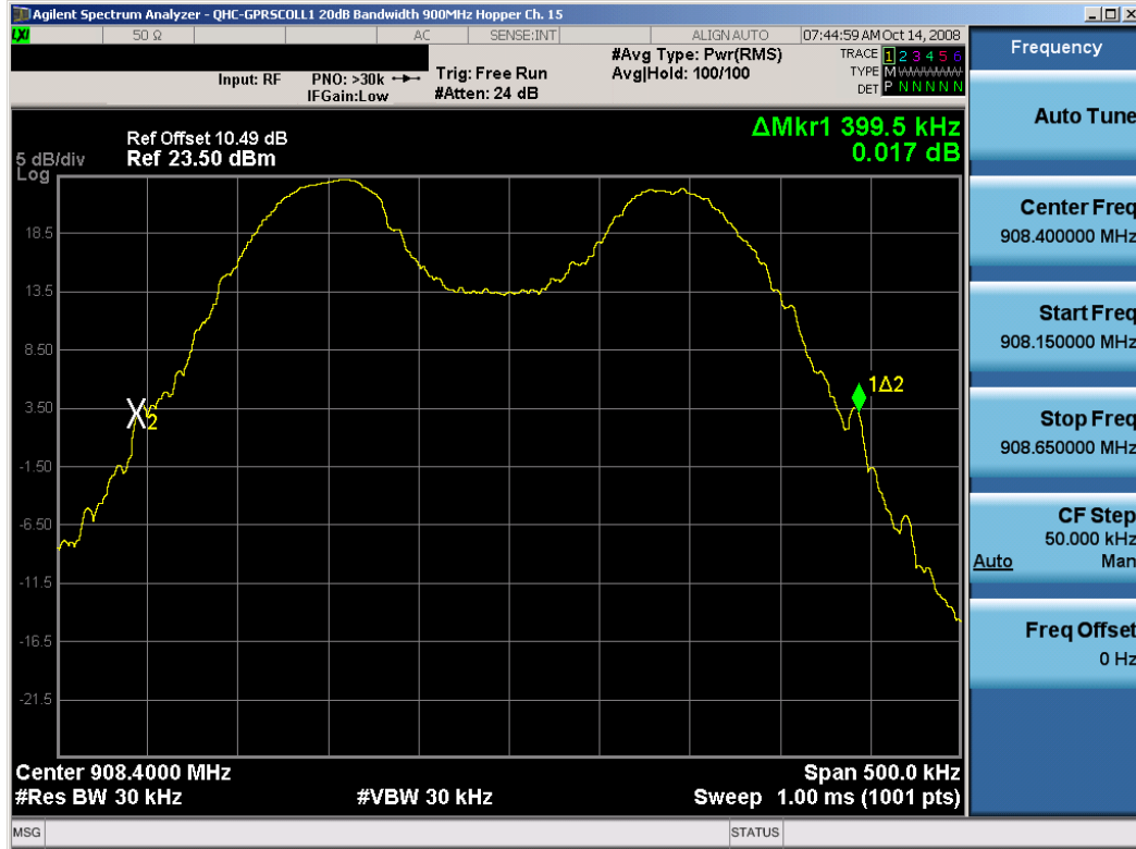
Plot 6-2. 20dB Bandwidth Plot (Ch. 15)
