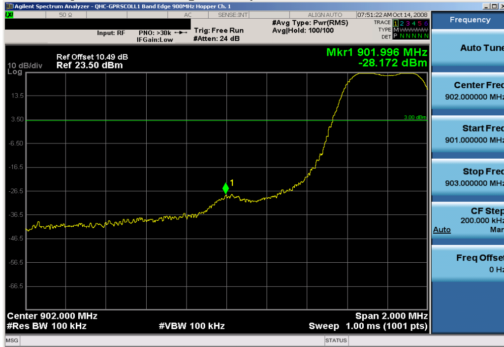
Plot 6-7. Lower Band Edge Plot (Ch. 1)
