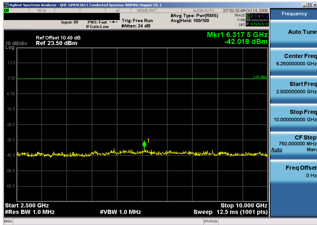
Plot 6-16. Conducted Spurious Plot (Ch. 1)
