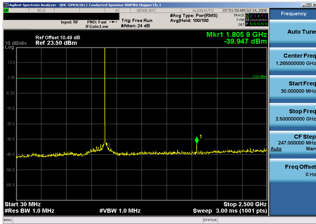
Plot 6-15. Conducted Spurious Plot (Ch. 1)
