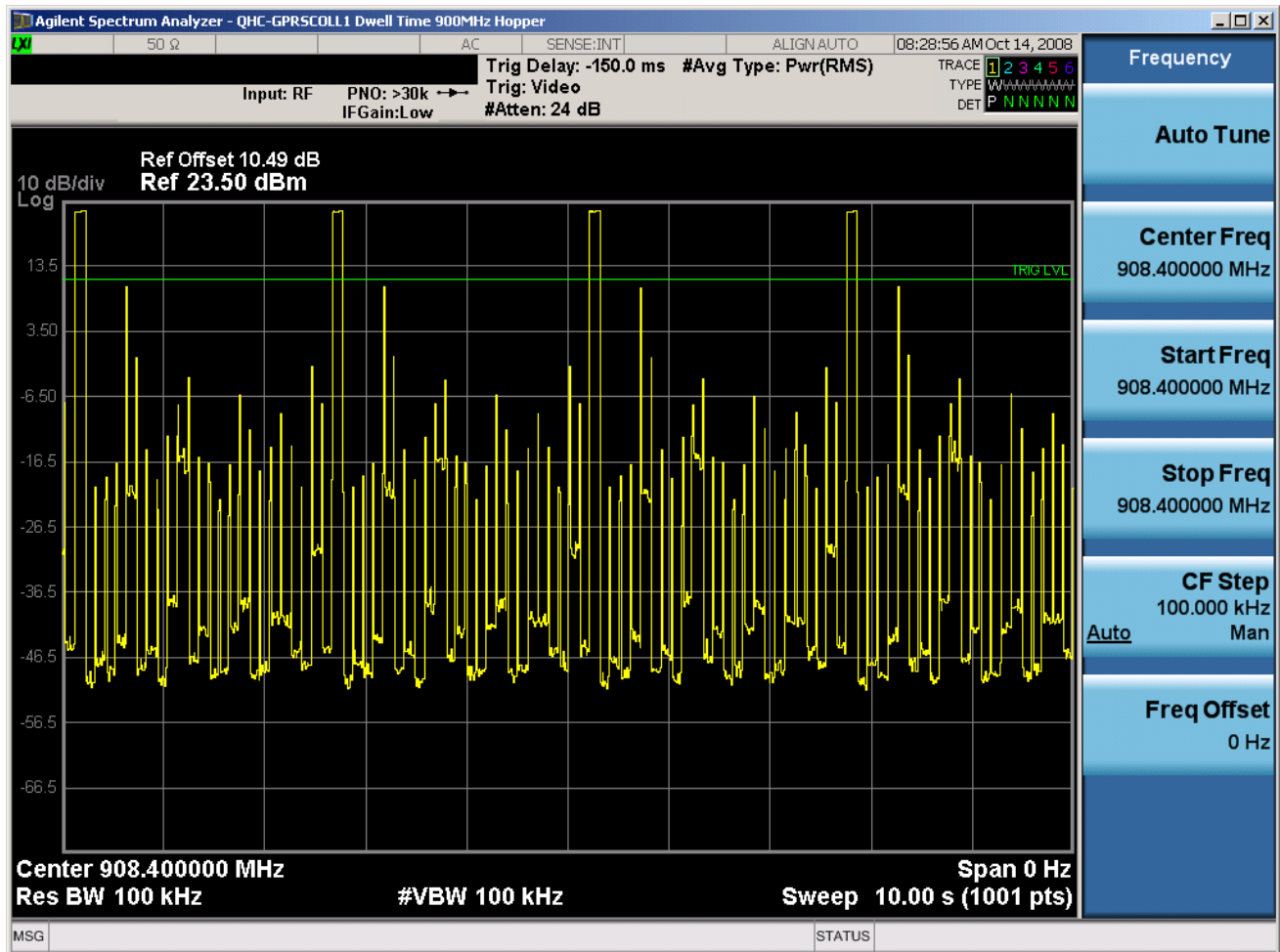
Plot 6-13. Time of Occupancy Plot
