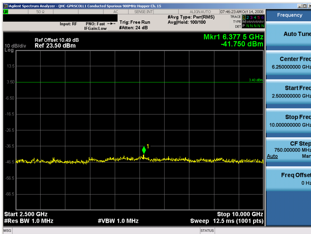
Plot 6-18. Conducted Spurious Plot (Ch. 15)
