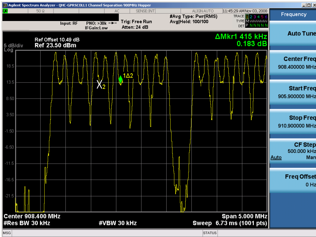
Plot 6-11. Channel Spacing Plot (Hopping Mode)
