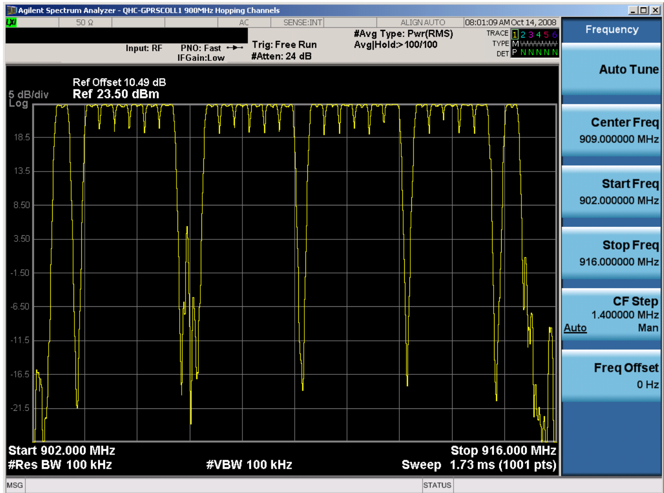
Plot 6-14. 900MHz Spectrum Channel Hopping Plot
