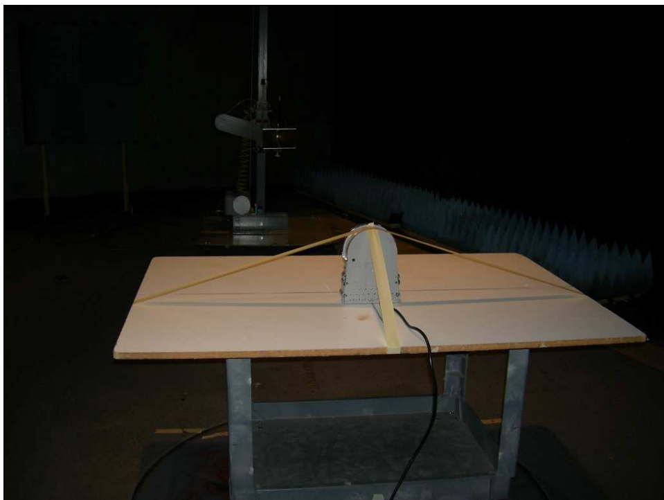
Figure 2: Test Setup Photograph – Radiated Emissions – EUT Installed in Meter
