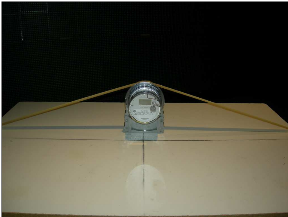
Figure 1: Test Setup Photograph – Radiated Emissions – EUT Installed in Meter
