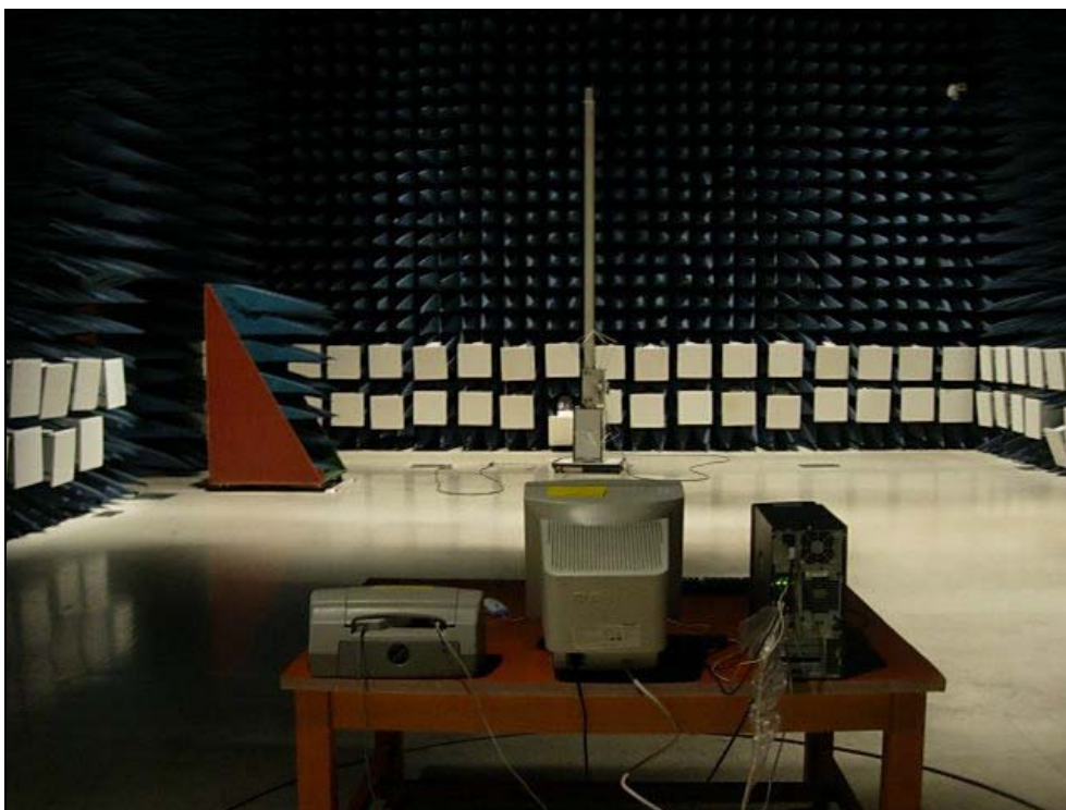
Radiated Disturbance<Rear>
