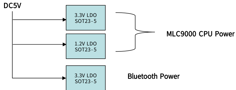
Power Block Diagram
