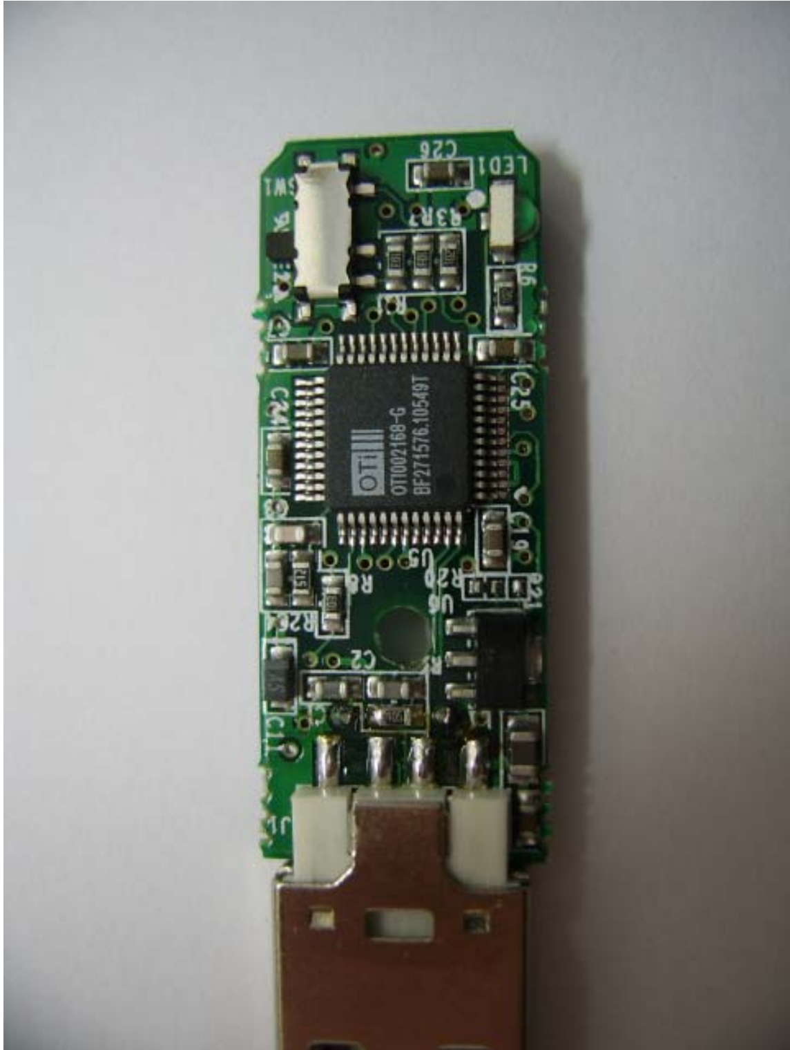
Board Front
