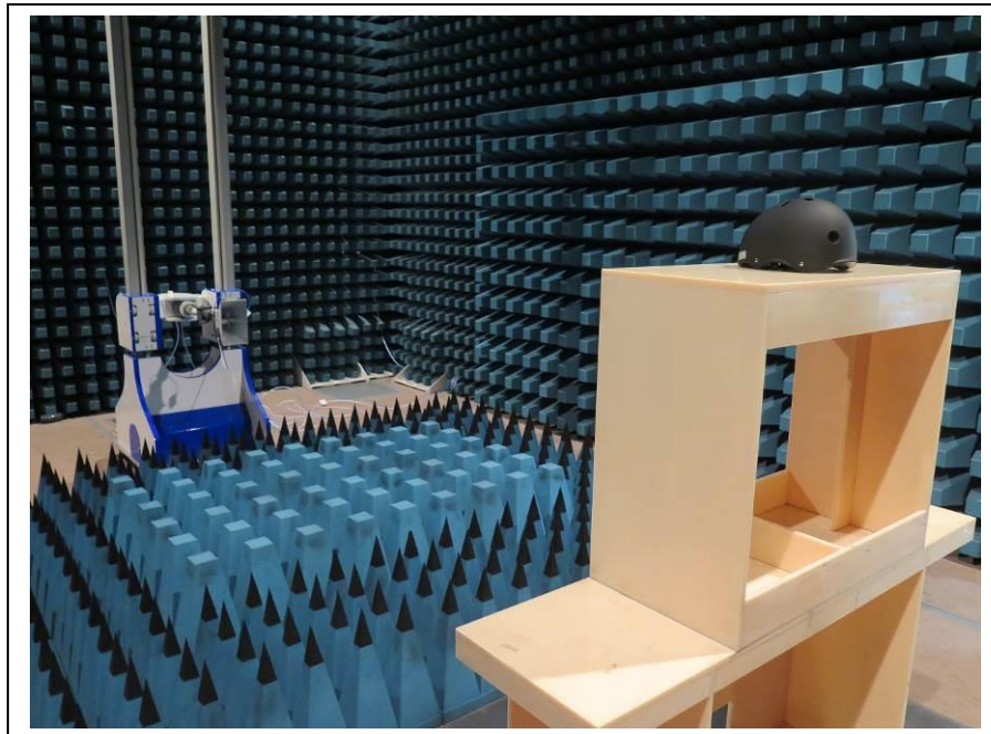
Above 1GHz
