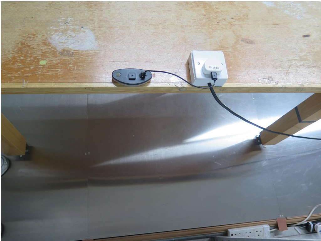
Line conducted emission (back view)
