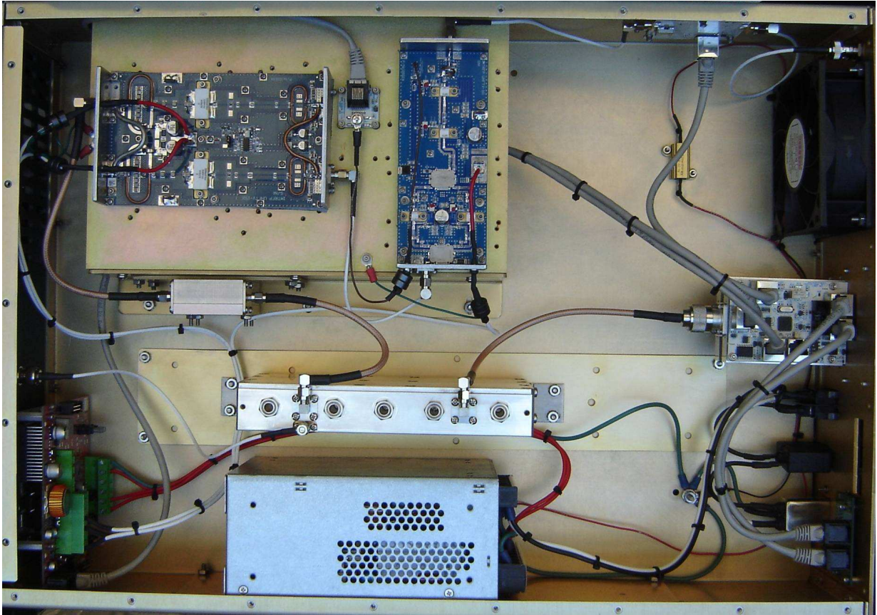
Power Amplifier (lids removed):
