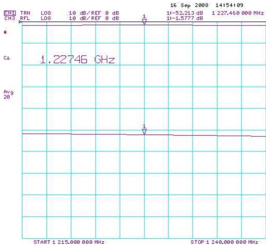
L2 band (1215-1240 MHz)
