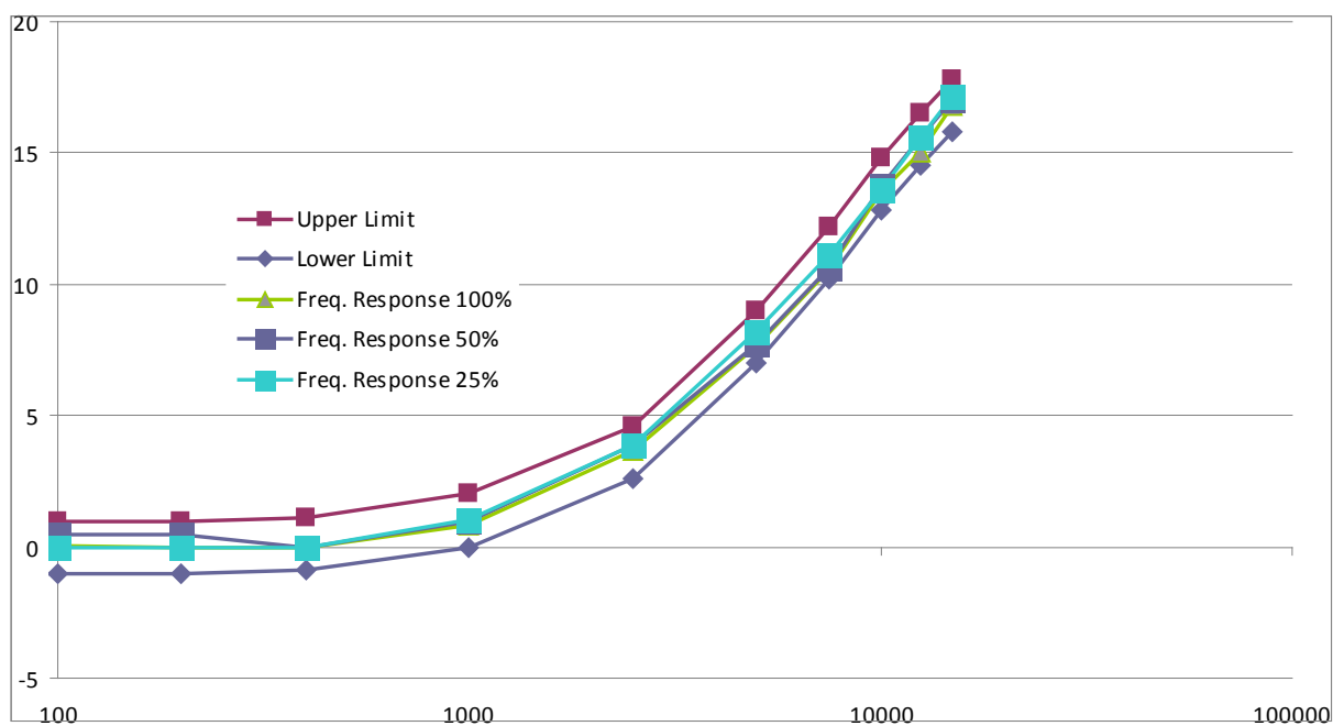
Figure 3: Audio Frequency Response (Mono) with 108.0MHz Carrier (25, 50, 100% Modulation)
