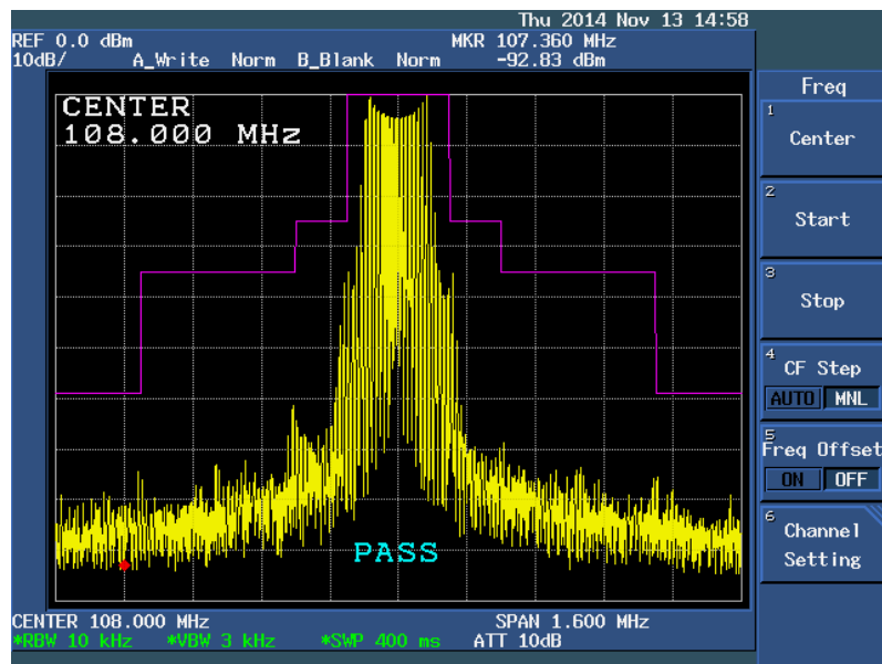
Figure 8: Occupied Bandwidth for Low and High Frequency Carriers
