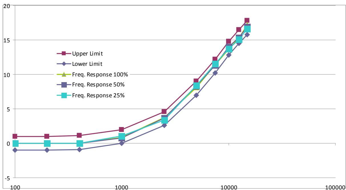
Figure 2: Audio Frequency Response (Mono) with 88.0MHz Carrier (25, 50, 100% Modulation)
