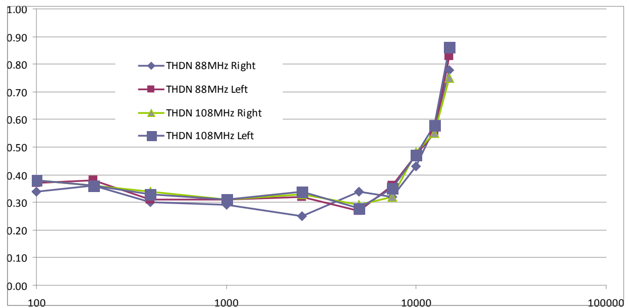
Figure 13: Audio Harmonic Distortion at 88.0 and 108.0MHz Carrier (Stereo)
