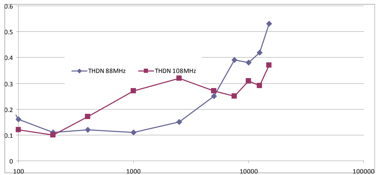
Figure 11: Audio Harmonic Distortion at 88.0 and 108.0MHz Carrier (Mono)
