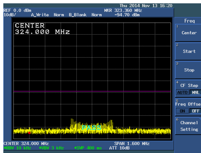
Figure 10: Spurious Emissions with 108.0MHz Carrier
