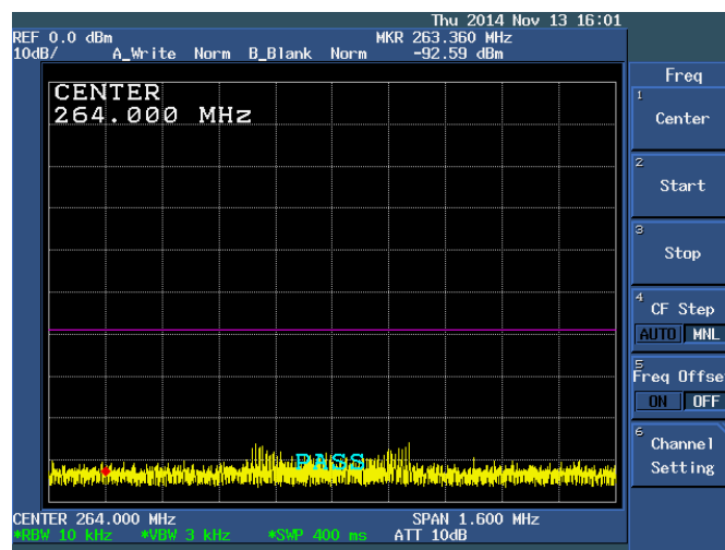
Figure 9: Spurious Emissions with 88.0MHz Carrier
