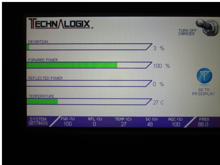
Figure 1: RF Output Level on Wattmeter and Transmitter Readout
