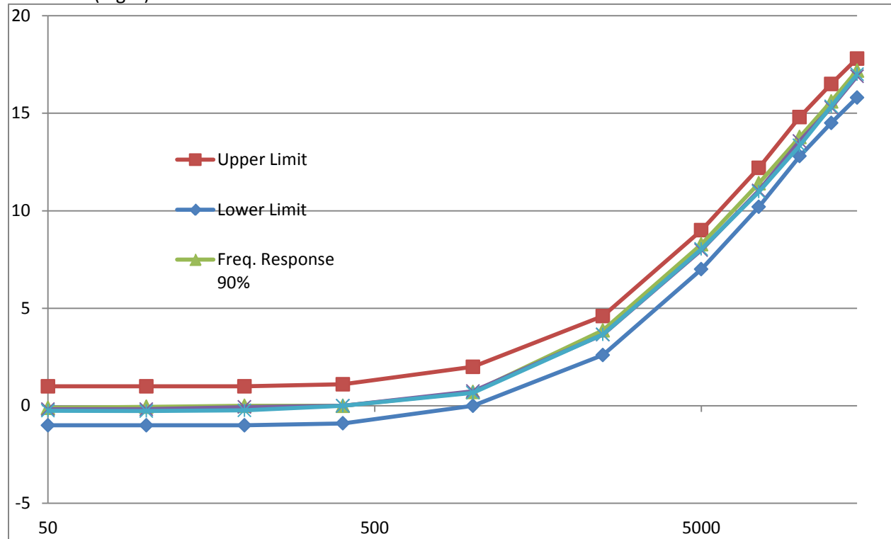
88.0 MHz (Right)
