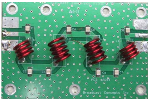
Lowpass Filter Construction (lid removed):
