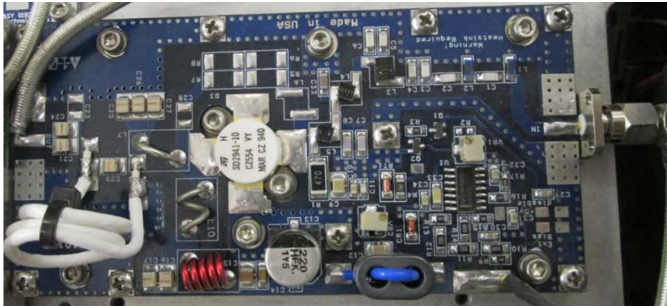
Power Amplifier Construction (lid removed):
