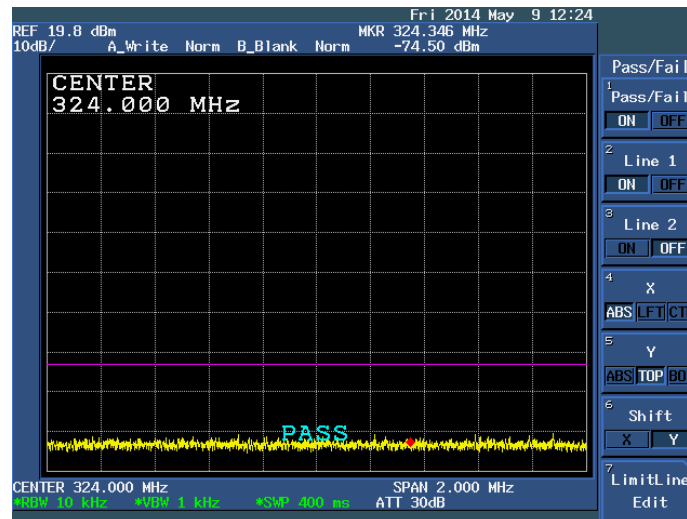
Figure 10: Spurious Emissions with 108.0MHz Carrier
