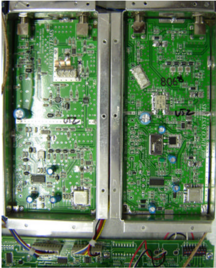
Internal view of Upconverter and Downconverter PCB:
