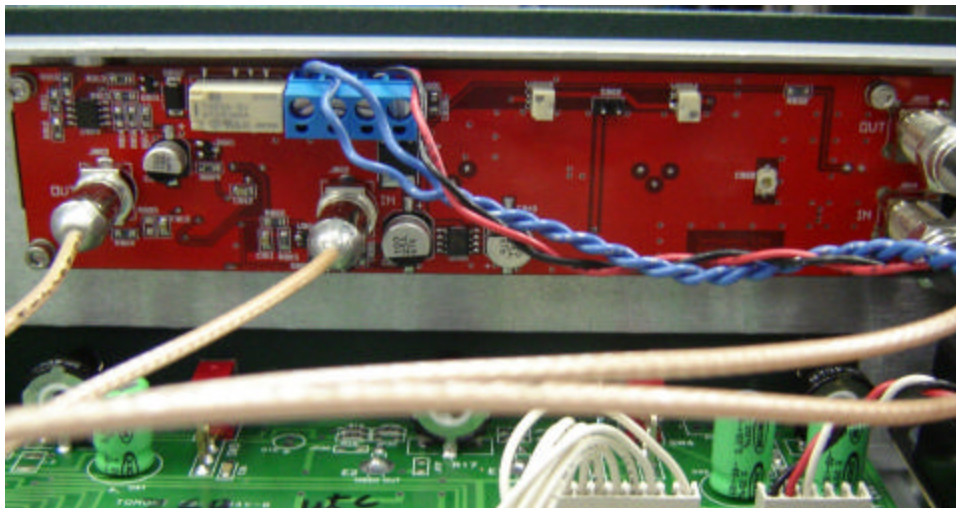
Bottom Layer of IF Precorrection PCB:
