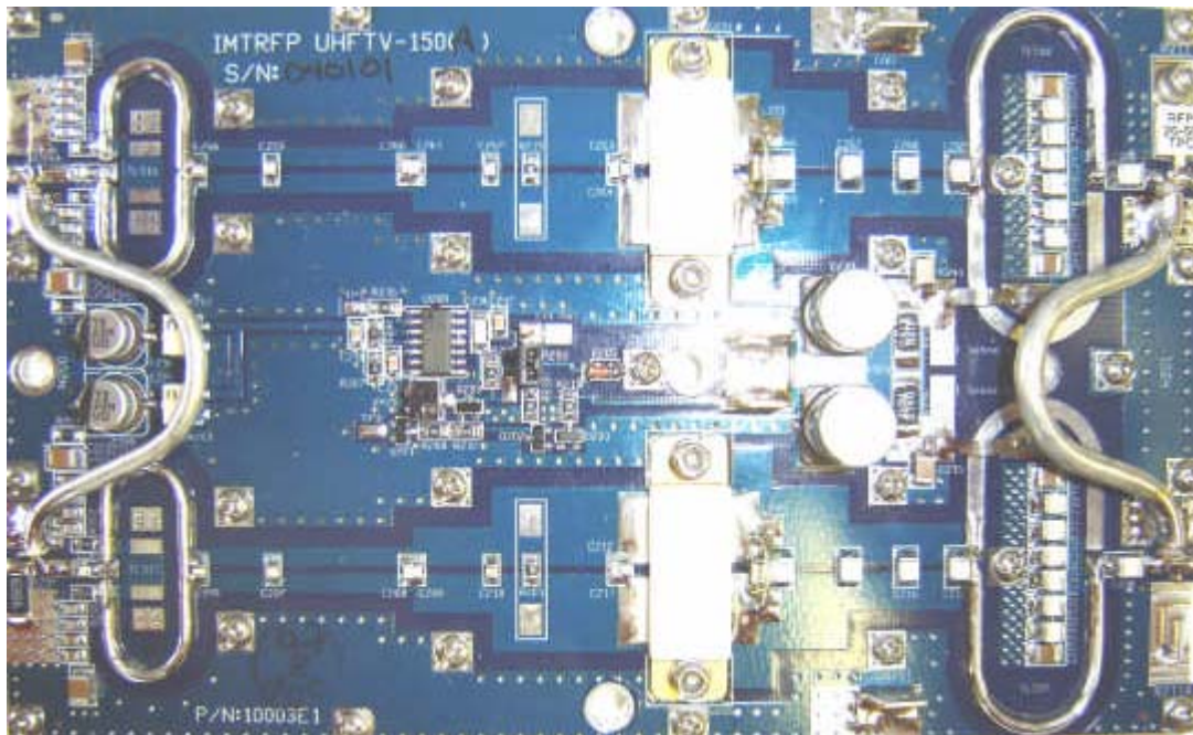
UHFTV-150 final (bottom side):
