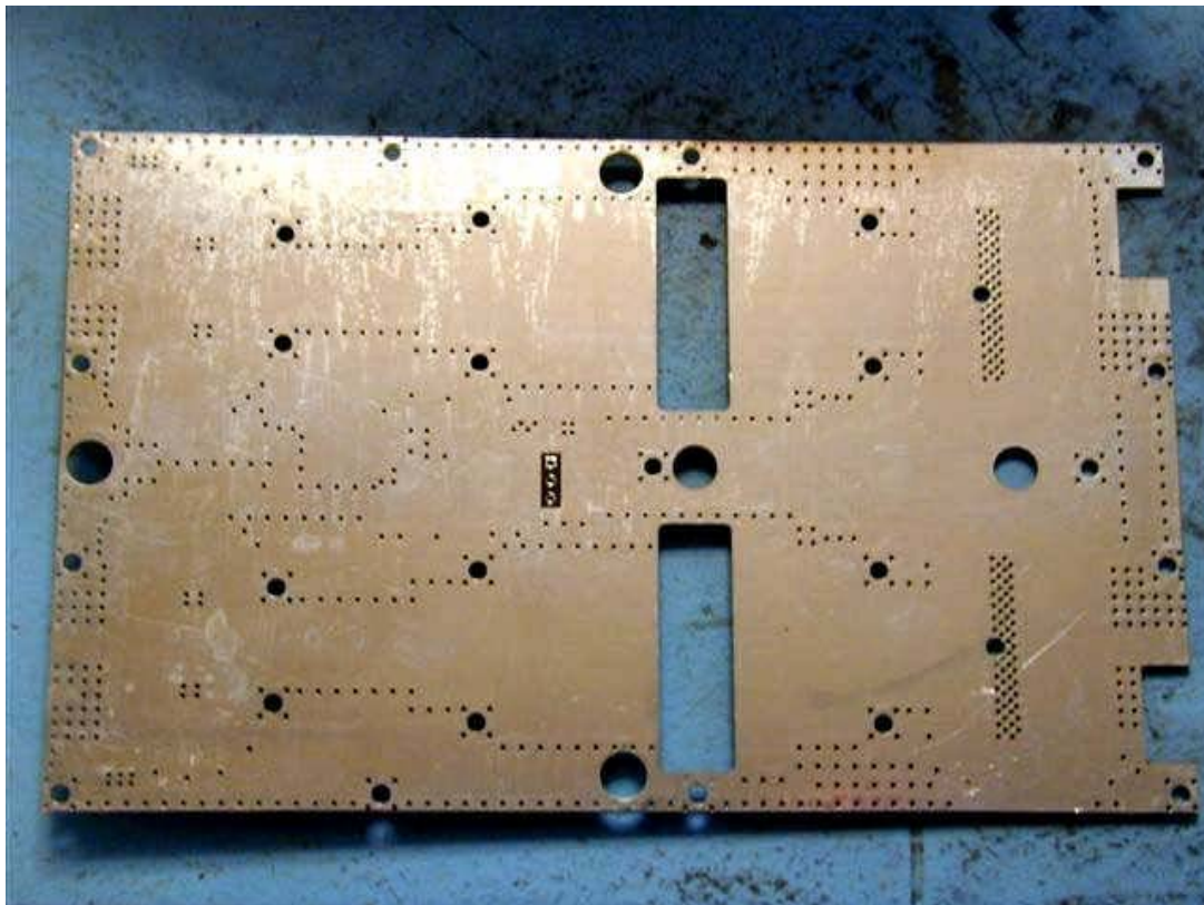
UHFTV-150 final (bottom side):
