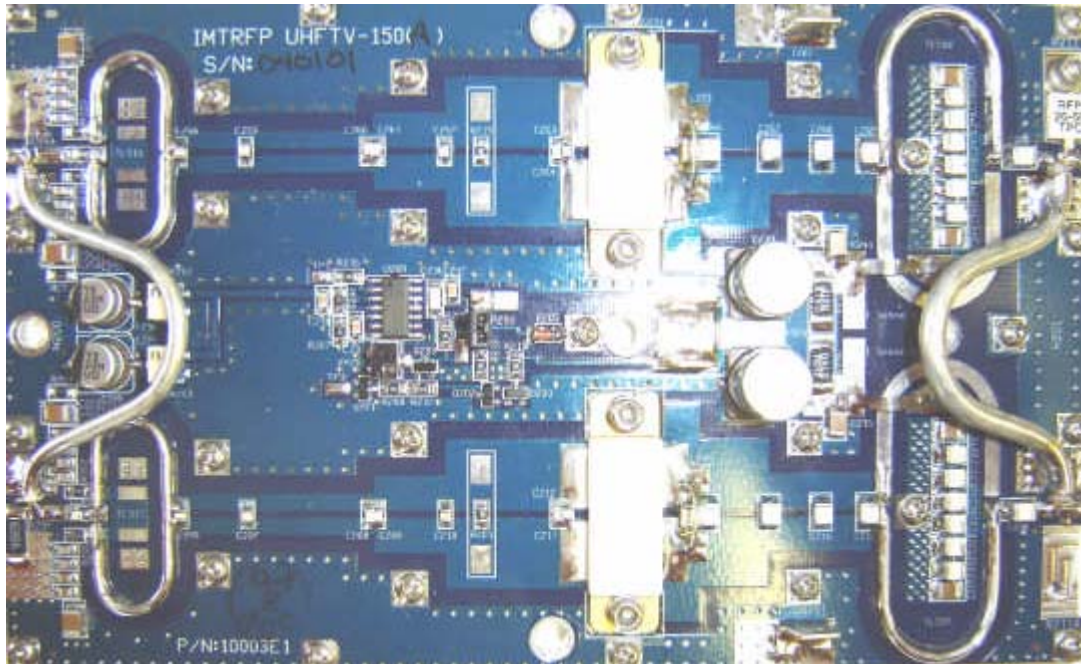
UHFTV-150 final (top side):
