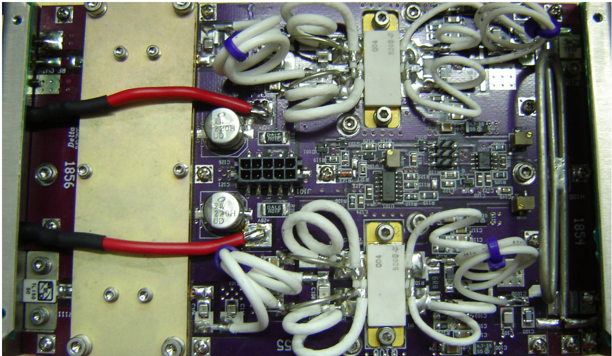
P400-VHF-H (component side with all components):
