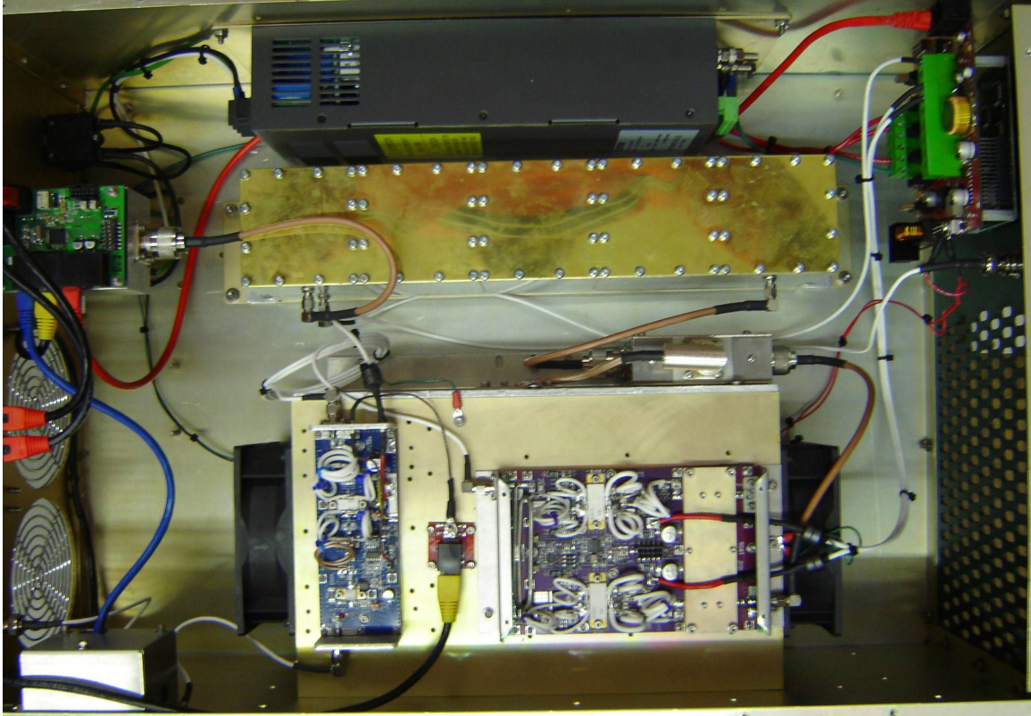
Internal Construction (amplifier pallet lids removed):
