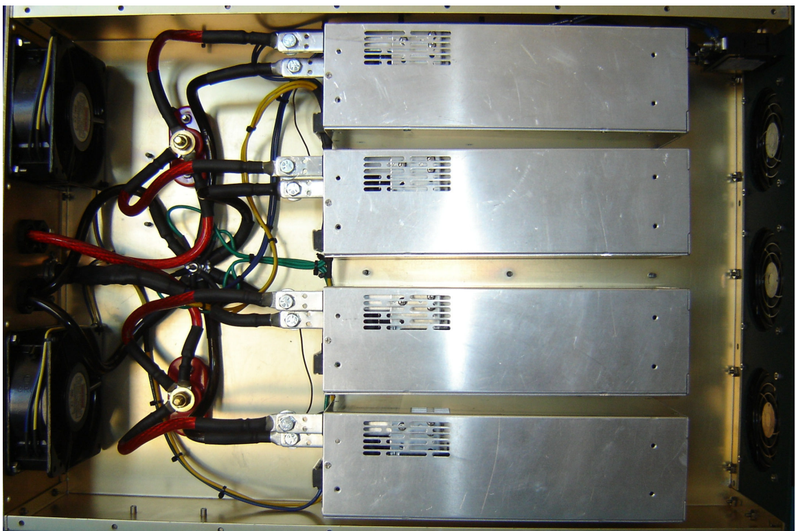
Power Supply Internal Construction:
