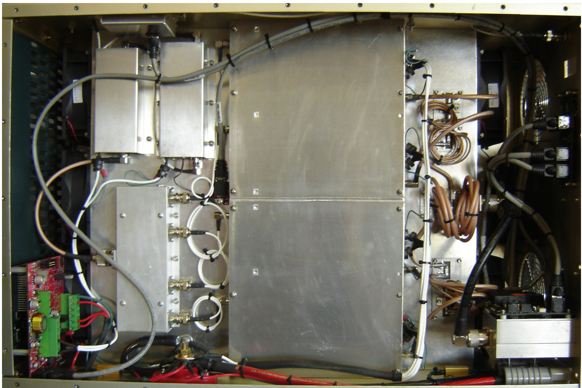
PA2 Internal Construction:
