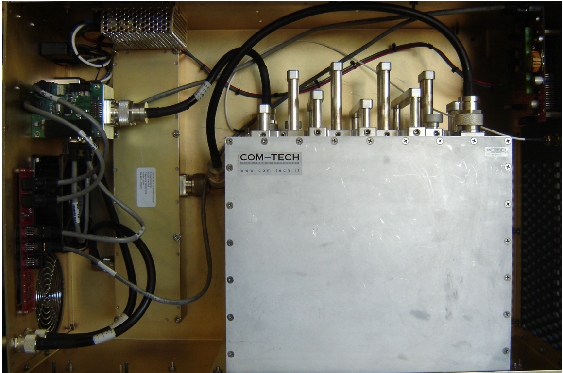
Combiner/Filter Box Internal Construction:
