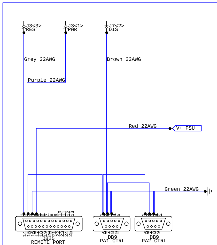
Combiner
