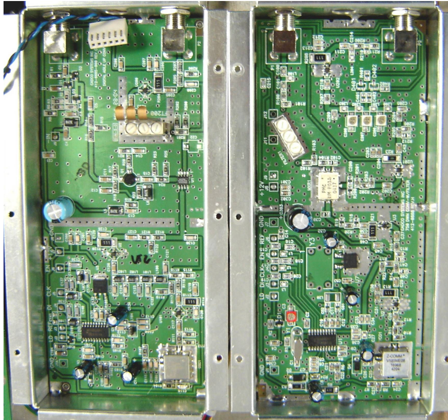
Internal view of Upconverter and Downconverter PCB:
